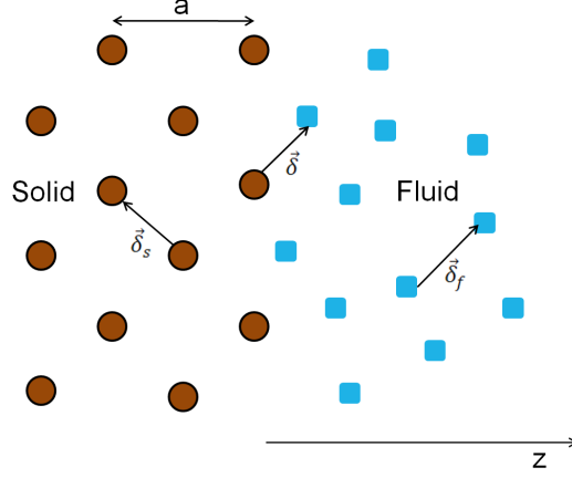
Figure 5.1. Cartoon of solid-fluid interface. Solid atoms are on the left and fluids are to the right. The interface is perpendicular to the z axis. Arrows denote the vectors used in the following equations.
