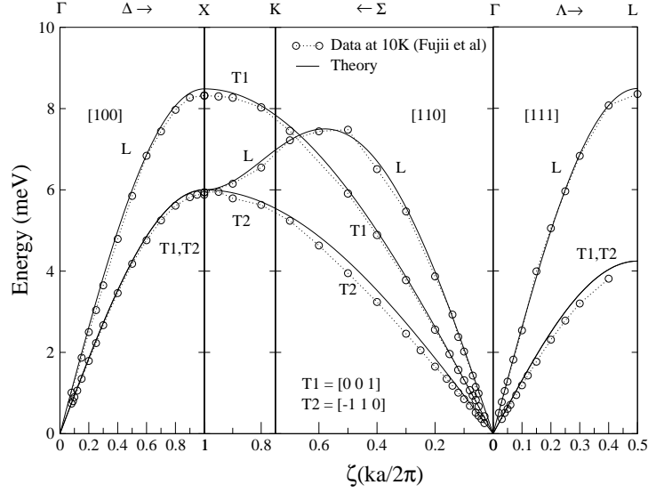
Figure 5.3. Phonon modes in solid Argon along the different symmetry lines of the FCC lattice. Experimental data taken from Fujii et al [8].
