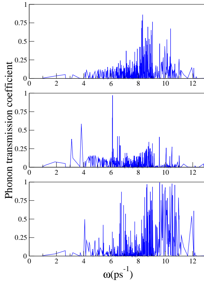
Figure 5.7. Phonon transmission coefficient \mathcal{T} at the interface between solid Argon and fluid Neon. The density and the temperature of the fluid are given by n = 0.0239\text{\AA}^{-3} and T = 54.345\text{K} , respectively.
