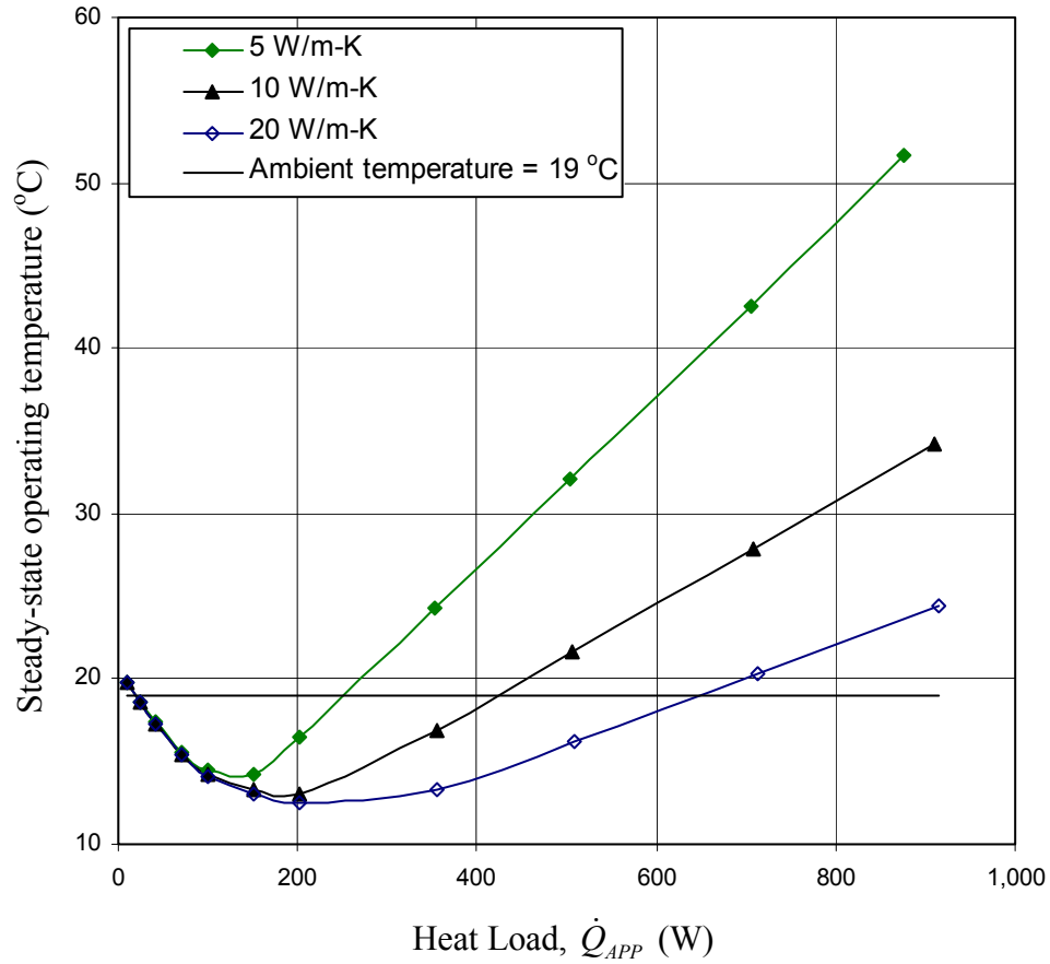
Fig. 6.23: Effect of external thermal conductance of the condenser on the steady-state operating temperature. ( T_{SINK} = 5^\circ\text{C} , T_{AMB} = 19^\circ\text{C} , and zero elevation)
