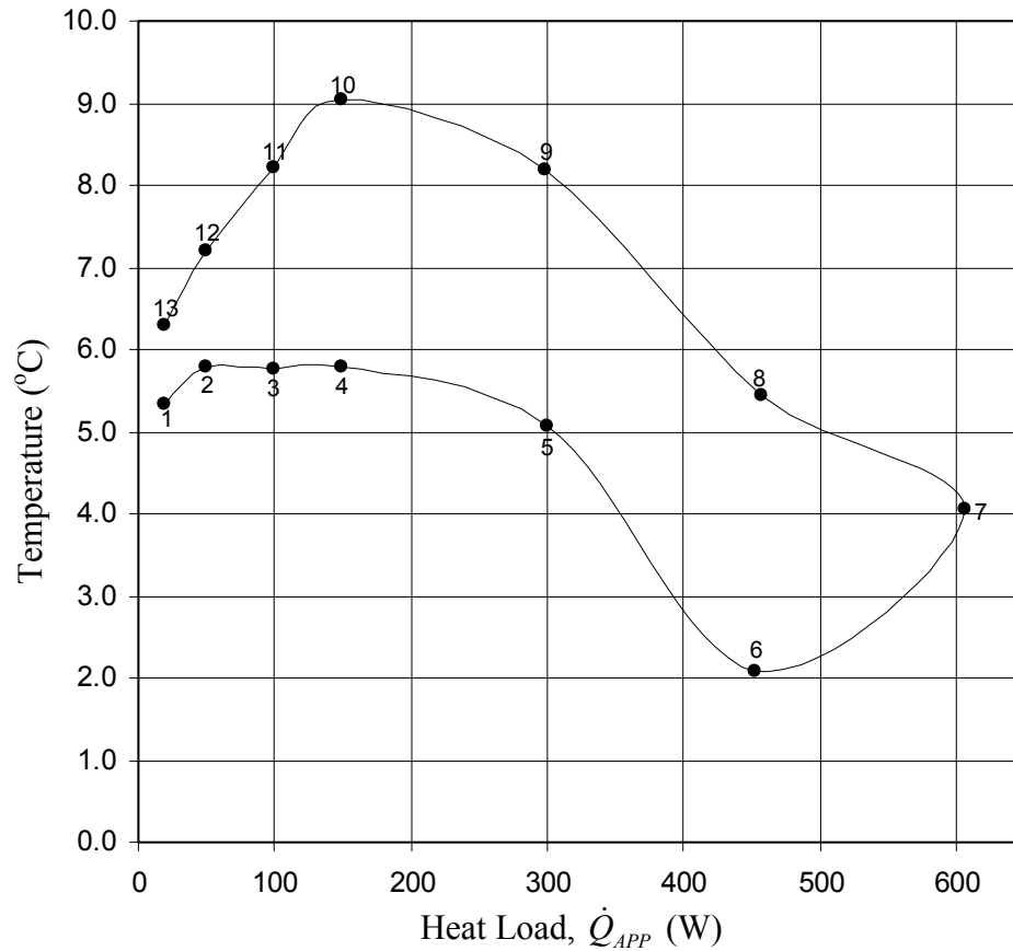
Fig. 7.20: Difference between the steady-state operating temperature and the fluid temperature exiting the liquid line as a function of heat load. ( T_{SINK}=5 °C, 3 ½-inch positive elevation, and insulation on the evaporator). The numbers represent the steps in the sequence of applying heat load.
