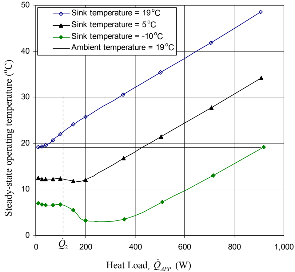
Fig. 6.17: Effect of sink temperature on the trend of steady-state operating temperature. ( T_{AMB} = 19^\circ\text{C} and 2-inch positive elevation)
