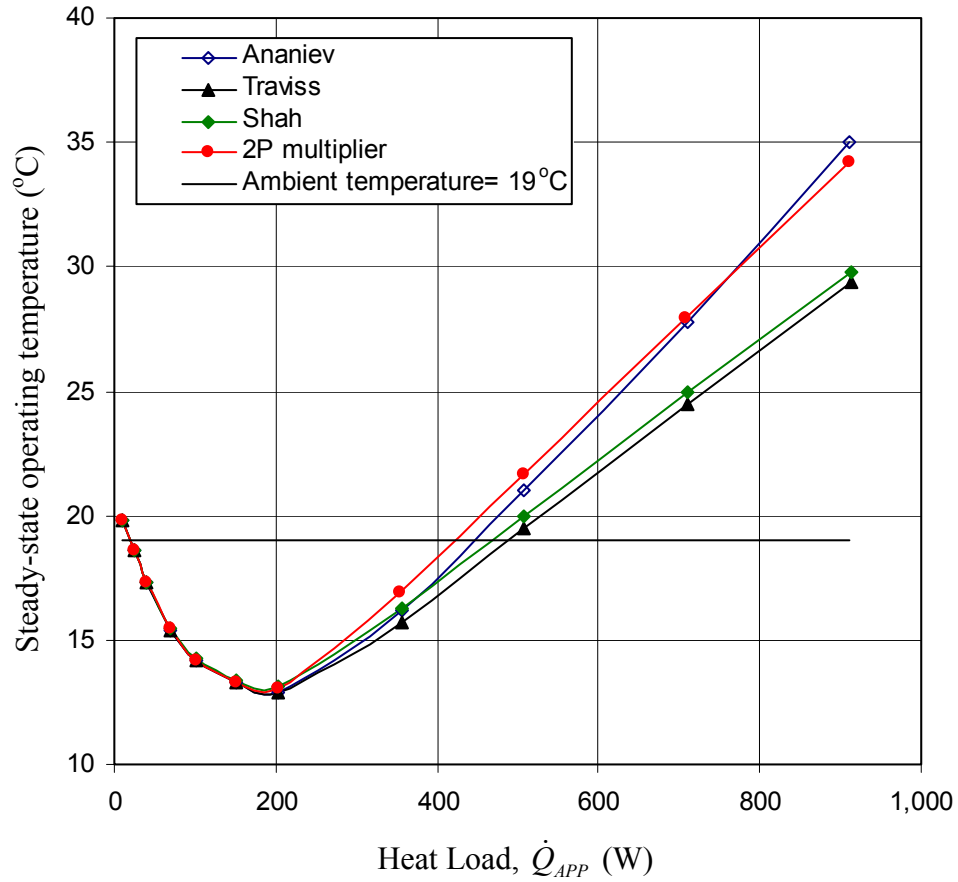
Fig. 6.24: Effect of two-phase heat transfer correlations on the steady-state operating temperature. ( T_{SINK} = 5^{\circ}\text{C} , T_{AMB} = 19^{\circ}\text{C} , zero elevation, and smooth annular correlation)
