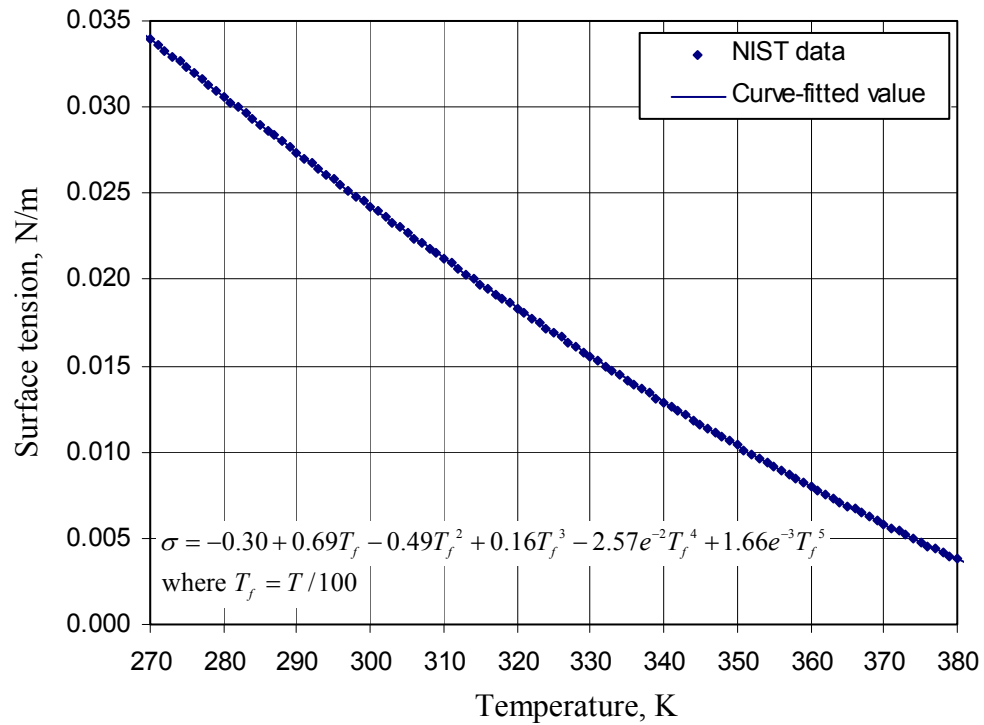
Fig. B.11: Surface tension of saturated ammonia.
