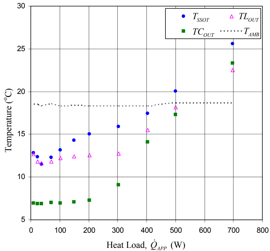
Fig. 7.11: Trends of steady-state operating temperature, temperatures exiting the liquid line and the condenser, and ambient temperature as functions of heat load. ( T_{SINK} = 5^\circ\text{C} , 5-inch positive elevation, and insulations on evaporator, reservoir, and vapor line)
