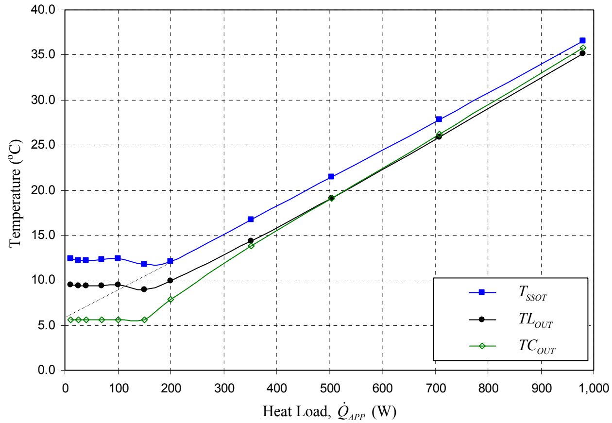
Fig. 6.8: Predicted trends of steady-state operating temperature and fluid temperatures exiting the liquid line and the condenser for the baseline configuration. ( T_{SINK} = 5^{\circ}\text{C} , T_{AMB} = 19^{\circ}\text{C} , and 2-inch positive elevation)
