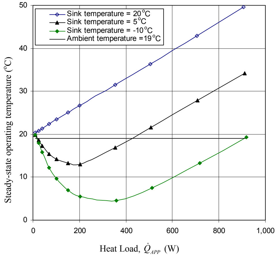
Fig. 6.16: Effect of sink temperature on the trend of steady-state operating temperature. ( T_{AMB} = 19^\circ\text{C} and zero elevation)
