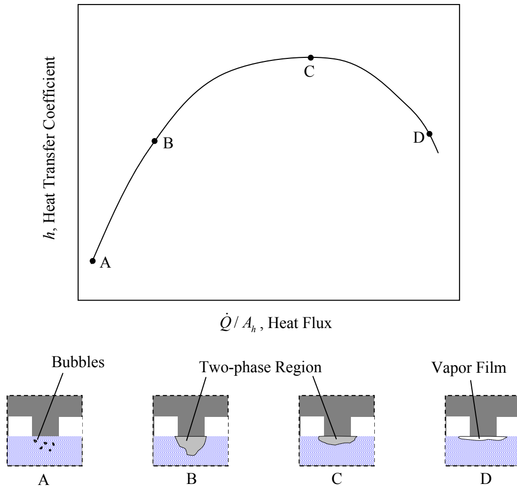
Fig. 5.7: Heat transfer coefficient vs. applied heat flux, and drawings of observations corresponding to different values of heat flux. (Adapted from Liao and Zhao, 1999)
