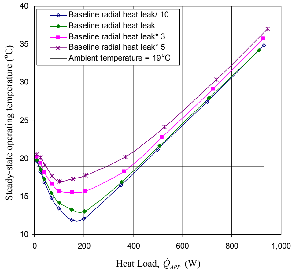
Fig. 6.27: Effect of radial heat leak on the steady-state operating temperature. ( T_{SINK} = 5^\circ\text{C} , T_{AMB} = 19^\circ\text{C} , zero elevation, and smooth annular correlation)
