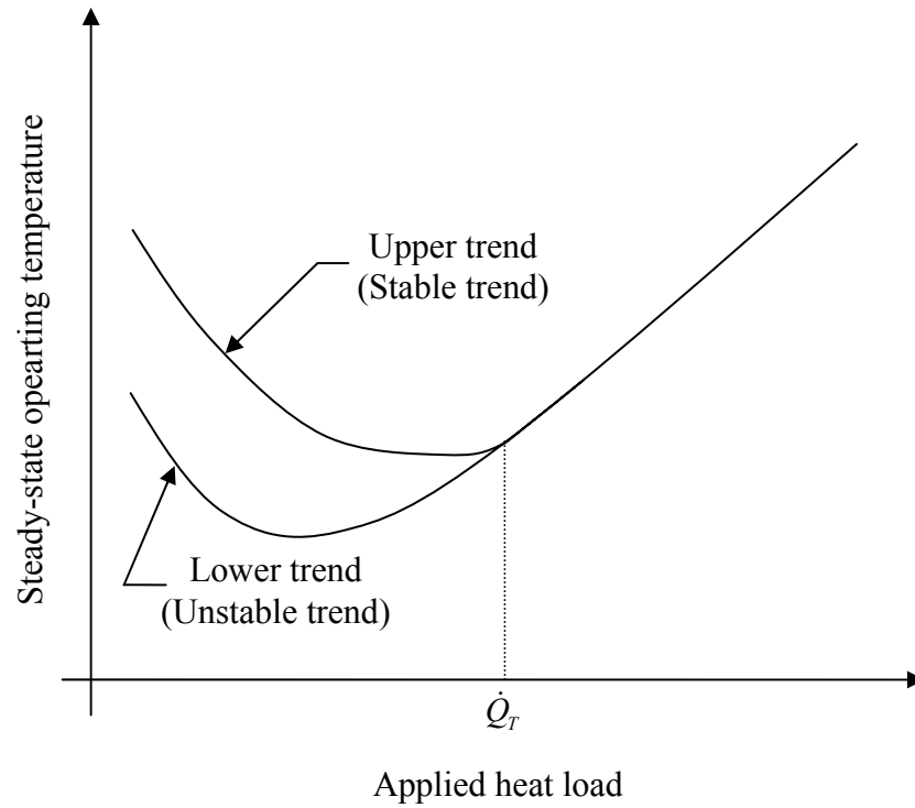
Fig. 2.4: Typical trend of steady-state operating temperature as a function of heat load when temperature hysteresis is observed.
