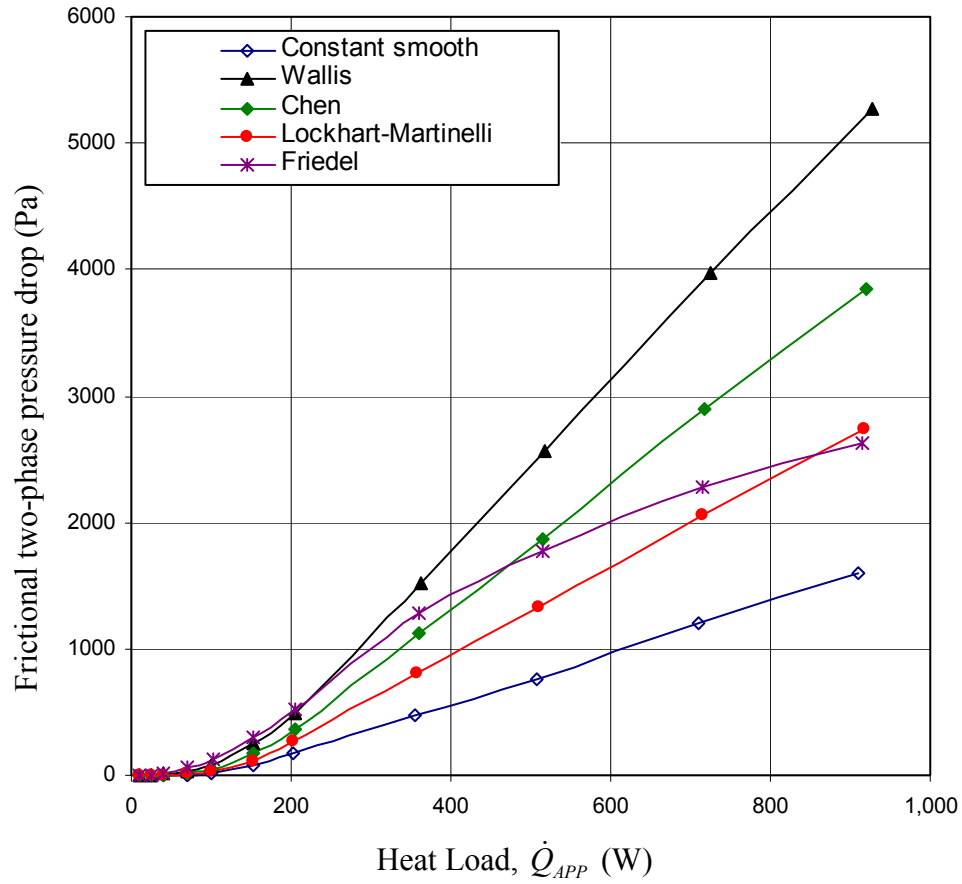
Fig. 6.29: Effect of two-phase pressure drop correlations on the frictional two-phase pressure drop. ( T_{SINK} = 5^\circ\text{C} , T_{AMB} = 19^\circ\text{C} , and Ananiev correlation)
