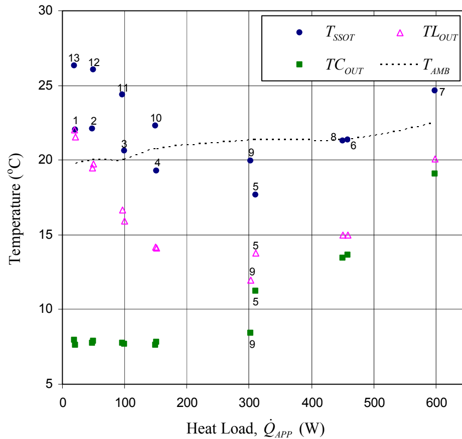
Fig. 7.15: Steady-state operating temperature, temperatures exiting the liquid line and condenser, and ambient temperature as functions of heat load. ( T_{SINK}=5 °C, 3 ½-inch adverse elevation, and insulation on the evaporator). The numbers represent steps in the sequence of applying heat load.
