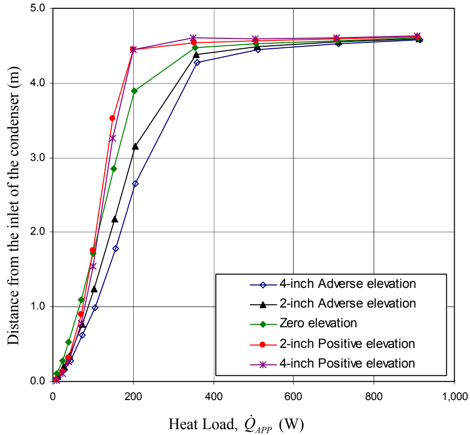
Fig. 6.21: Effect of elevation on the location of the liquid-vapor interface in the condenser. ( T_{SINK} = 5\text{ }^{\circ}\text{C} and T_{AMB} = 19\text{ }^{\circ}\text{C} )
