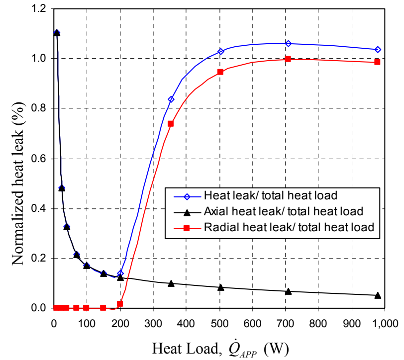
Fig. 6.14: Normalized total heat leak, axial heat leak, and radial heat leak as functions of heat load. ( T_{SINK} = 5^\circ\text{C} , T_{AMB} = 19^\circ\text{C} , and 2-inch positive elevation)
