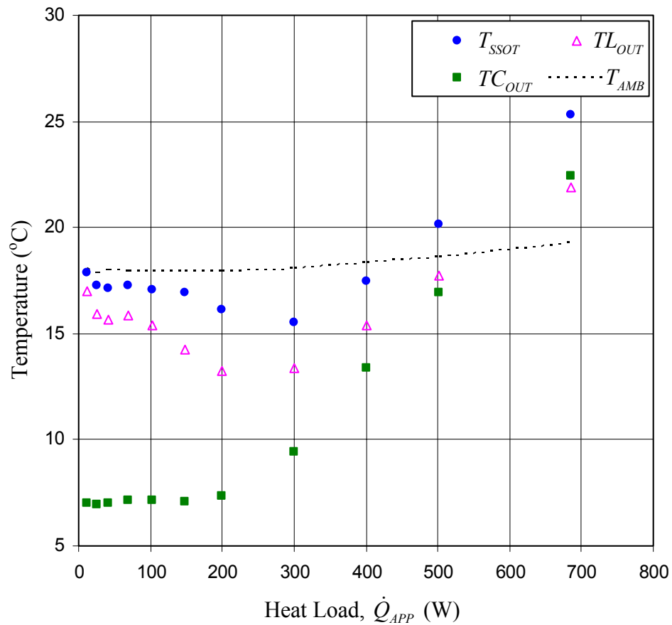
Fig. 7.10: Trends of steady-state operating temperature, temperatures exiting the liquid line and the condenser, and ambient temperature as functions of heat load. ( T_{SINK} = 5 °C, 3-inch positive elevation, and insulations on evaporator, reservoir, and vapor line)
