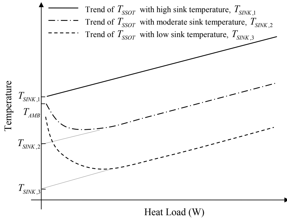
Fig. 4.4: Effect of sink temperature on steady-state operating temperature. (Ambient temperature is held constant at T_{AMB} .)
