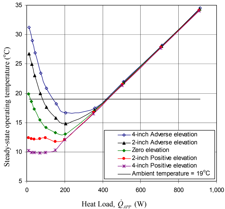
Fig. 6.20: Effect of elevation on the trend of steady-state operating temperature. ( T_{SINK} = 5\text{ }^{\circ}\text{C} and T_{AMB} = 19\text{ }^{\circ}\text{C} )
