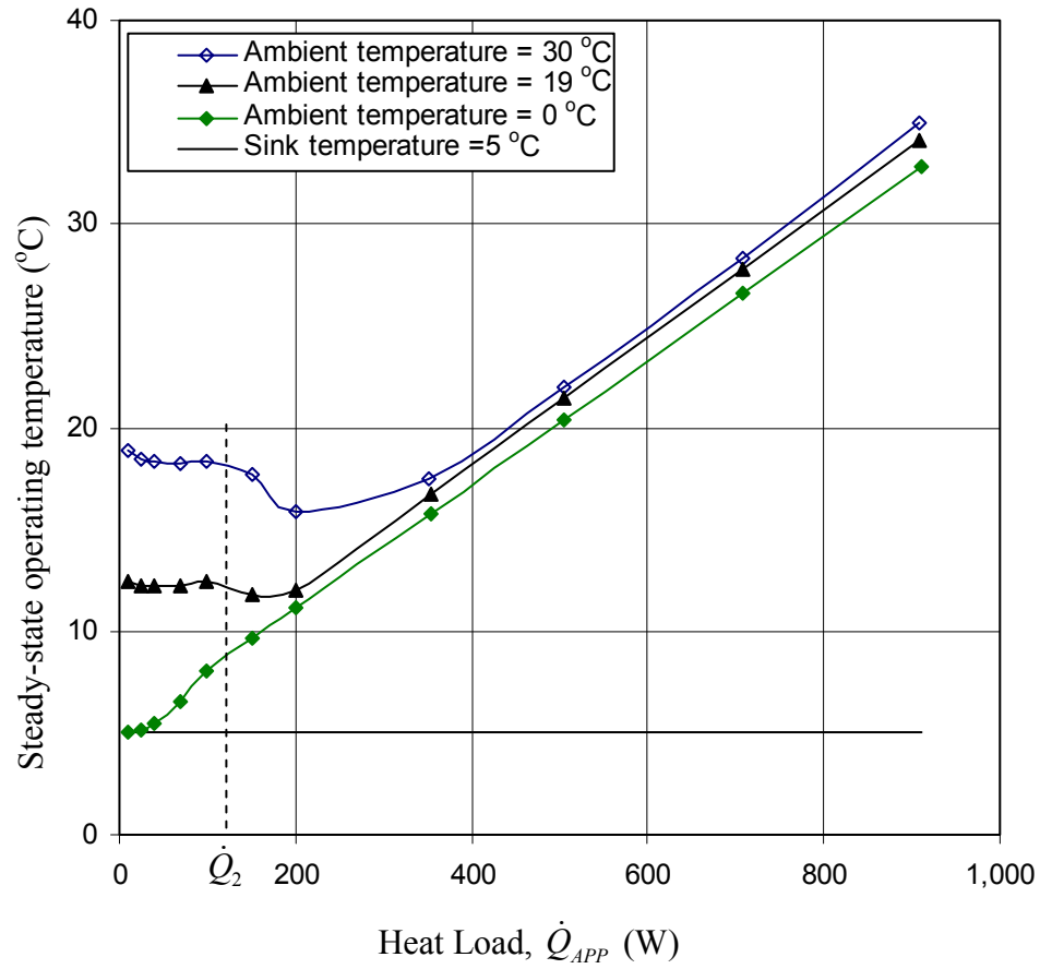
Fig. 6.19: Effect of ambient temperature on the trend of steady-state operating temperature. ( T_{SINK} = 5 °C and 2-inch positive elevation)
