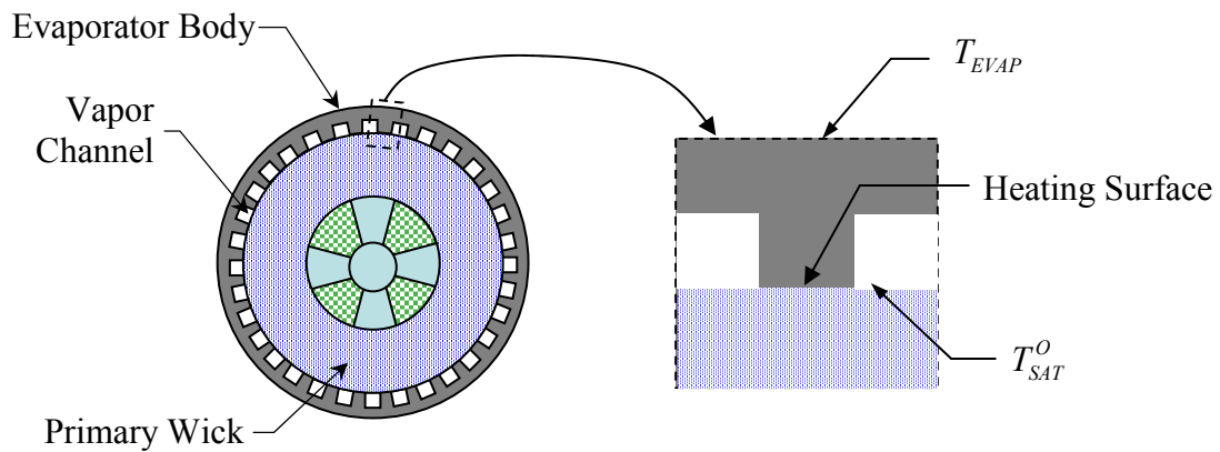
Fig. 5.6: A magnified drawing of the heating surface.
