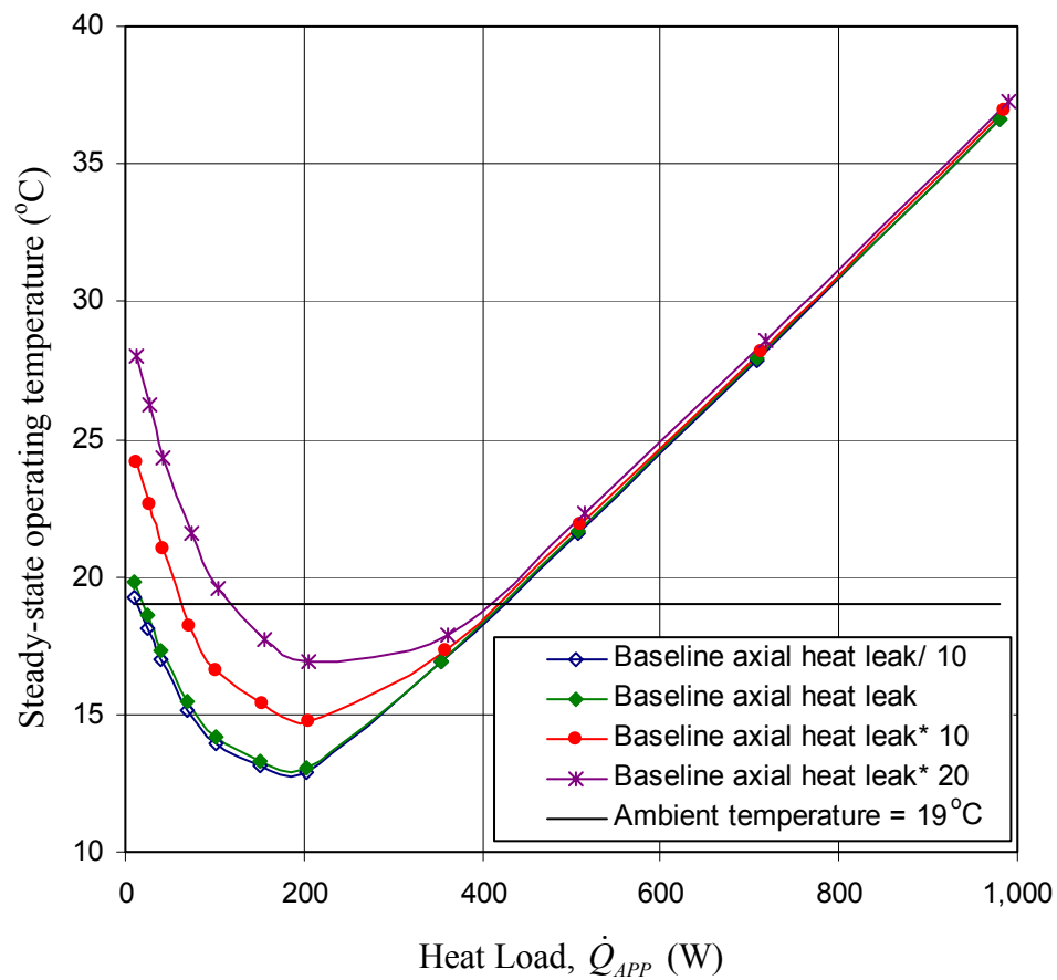
Fig. 6.26: Effect of axial heat leak on the steady-state operating temperature. ( T_{SINK} = 5^\circ\text{C} , T_{AMB} = 19^\circ\text{C} , zero elevation, and smooth annular correlation)
