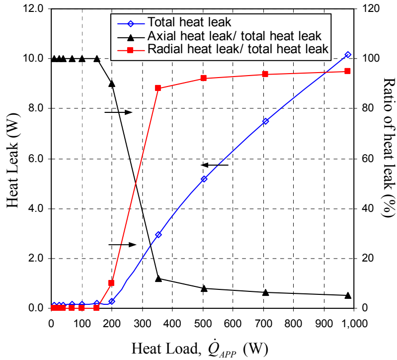
Fig. 6.13: Total heat leak and the ratios of axial heat leak and radial heat leak to total heat leak as functions of heat load. ( T_{SINK} = 5^\circ\text{C} , T_{AMB} = 19^\circ\text{C} , and 2-inch positive elevation)
