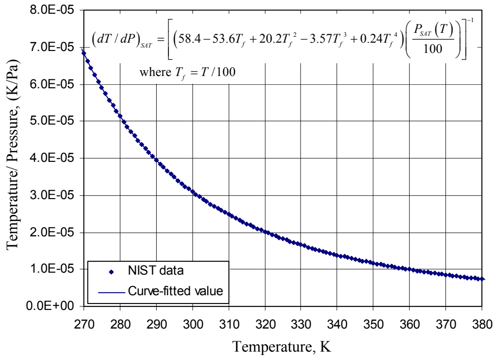
Fig. B.2: Temperature change/ Pressure change of saturated ammonia.
