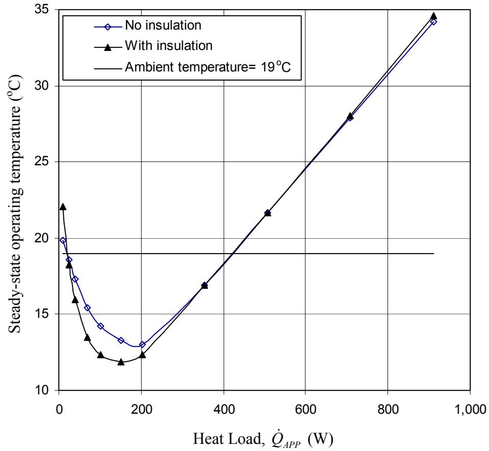
Fig. 6.30: Effect of insulation of the reservoir on the steady-state operating temperature. ( T_{SINK} = 5^\circ\text{C} , T_{AMB} = 19^\circ\text{C} , and zero elevation)
