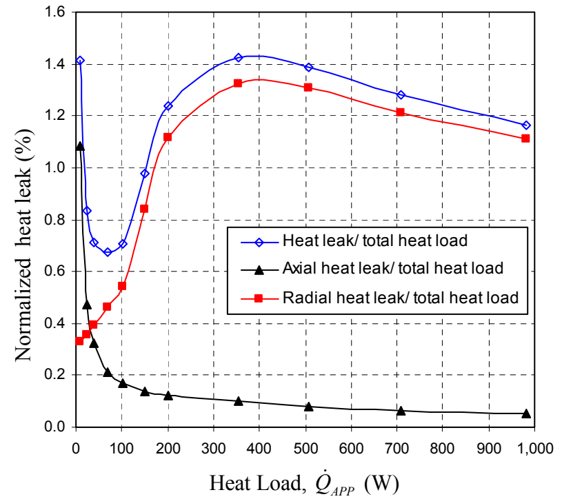
Fig. 6.6: Normalized total heat leak, axial heat leak, and radial heat leak as functions of heat load. ( T_{SINK} = 5^\circ\text{C} , T_{AMB} = 19^\circ\text{C} , and zero elevation)
