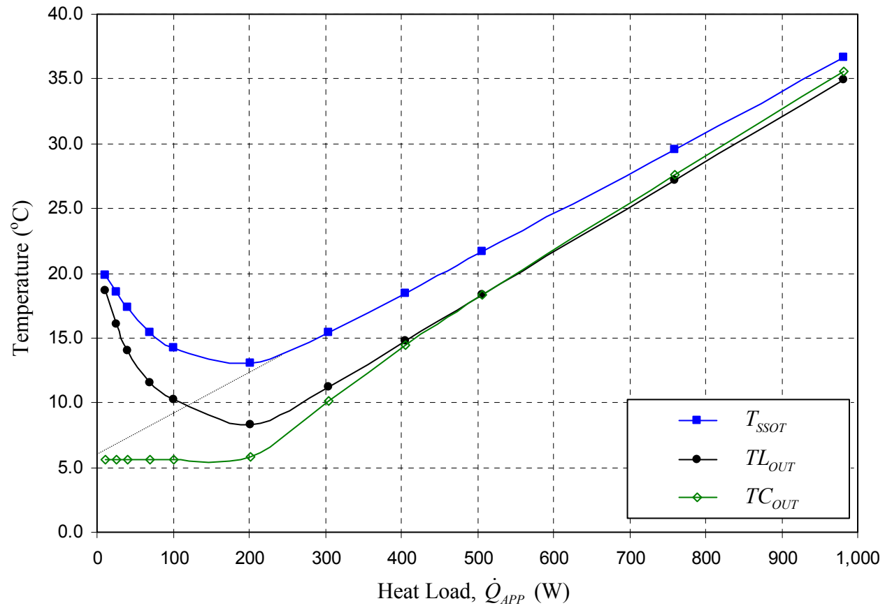
Fig. 6.1: Predicted trends of steady-state operating temperature and fluid temperatures exiting the liquid line and the condenser for the baseline configuration. ( T_{SINK} = 5^{\circ}\text{C} , T_{AMB} = 19^{\circ}\text{C} , and zero elevation)
