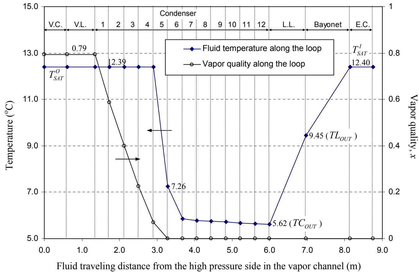
Fig. 6.15: Temperature and vapor quality of the fluid flow along the loop starting from the high pressure side in the vapor channel. ( T_{SINK} = 5\text{ }^{\circ}\text{C} , T_{AMB} = 19\text{ }^{\circ}\text{C} , 2-inch positive elevation, and \dot{Q}_{APP} = 100.17\text{ W} )
