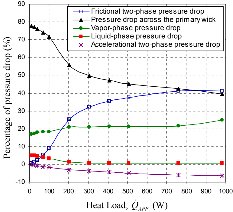
Fig. 6.2: Ratios of component pressure drops to total pressure drop as functions of heat load. ( T_{SINK} = 5^\circ\text{C} , T_{AMB} = 19^\circ\text{C} , zero elevation, and constant smooth correlation)
