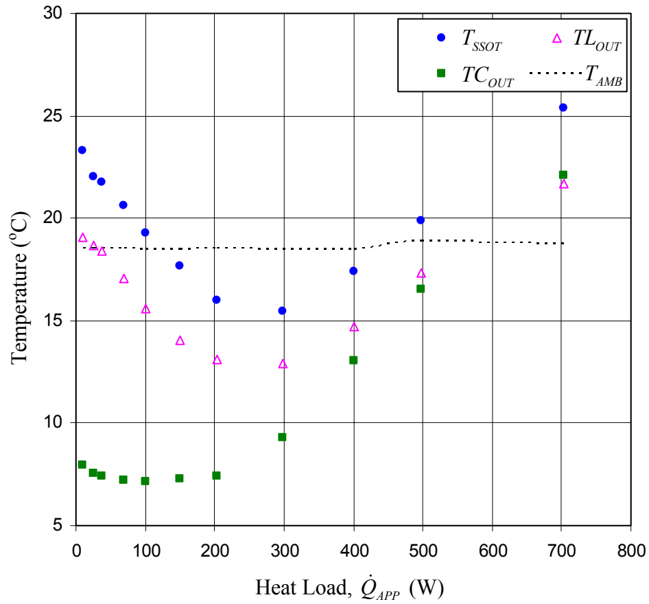
Fig. 7.8: Trends of steady-state operating temperature, temperatures exiting the liquid line and the condenser, and ambient temperature as functions of heat load. ( T_{SINK} = 5^\circ\text{C} , zero elevation, and insulations on evaporator, reservoir, and vapor line)
