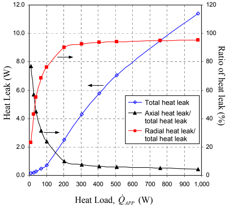
Fig. 6.5: Total heat leak and the ratios of axial heat leak and radial heat leak as functions of heat load. ( T_{SINK} = 5^\circ\text{C} , T_{AMB} = 19^\circ\text{C} , and zero elevation)
