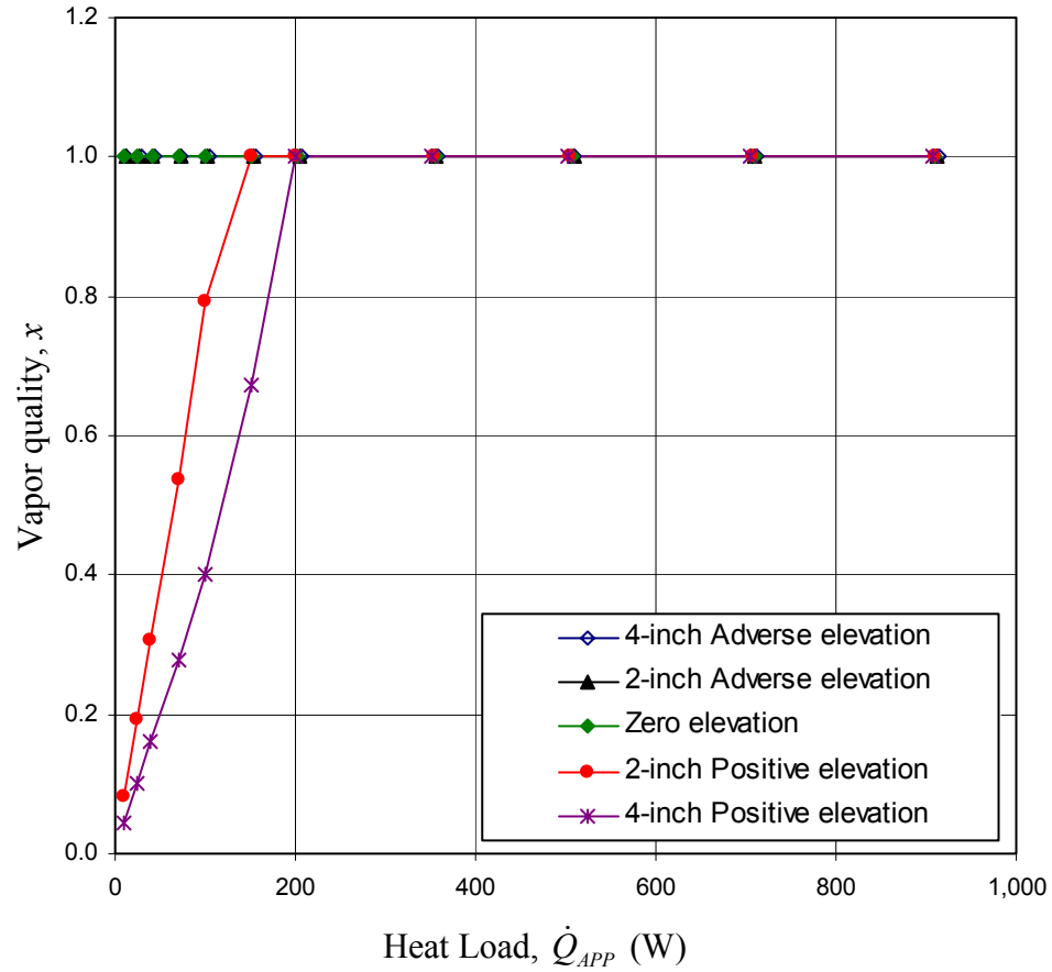
Fig. 6.22: Effect of elevation on the vapor quality exiting the vapor channel. ( T_{SINK} = 5^\circ\text{C} and T_{AMB} = 19^\circ\text{C} )
