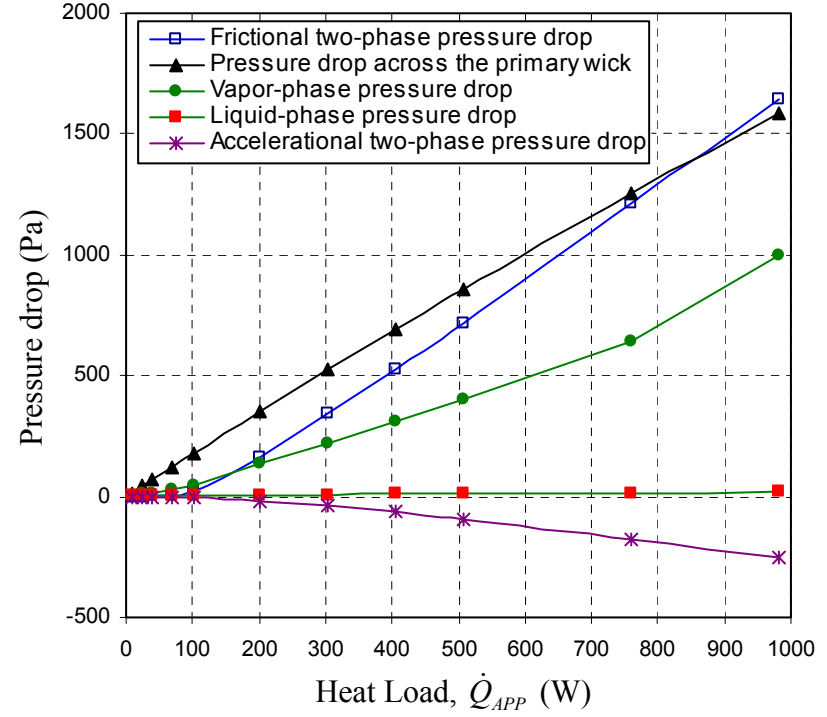
Fig. 6.3: Component pressure drops as functions of heat load. ( T_{SINK} = 5^\circ\text{C} , T_{AMB} = 19^\circ\text{C} , zero elevation, and constant smooth correlation)
