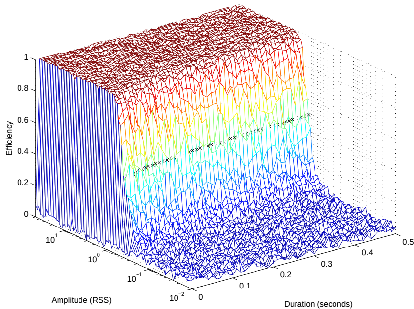
Figure G.16. BlockNormal efficiency to exponentially decaying harmonic oscillators of 16 Hz with varying amplitude and duration (shown as a 3-dimensional surface) [const. magnitude].
