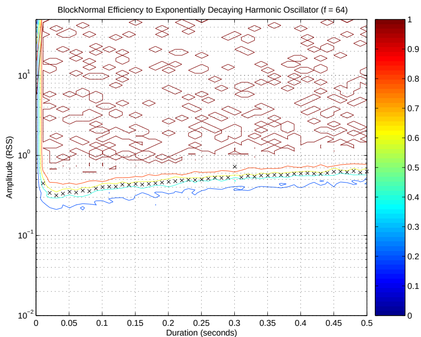
Figure E.26. BlockNormal efficiency to exponentially decaying harmonic oscillators of 64 Hz with varying amplitude and duration (shown as a contour plot).
