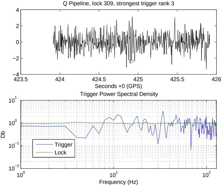
Figure D.9. Third strongest Q Pipeline trigger from all white noise data segments.
