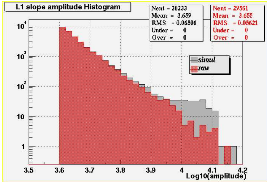
Figure 4.3. L1 measured slope frequency on S1 raw data with and without simulations. Image courtesy of Laura Cadonati for the LIGO Burst Group [5].
