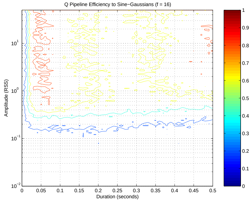
Figure 8.6. Q Pipeline efficiency to 16 Hz sine-Gaussians with varying amplitude and duration (shown as a contour plot) [const. magnitude].
