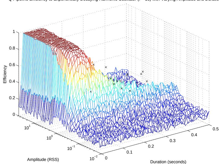
Figure E.23. Q Pipeline efficiency to exponentially decaying harmonic oscillators of 16 Hz with varying amplitude and duration (shown as a 3-dimensional surface).
