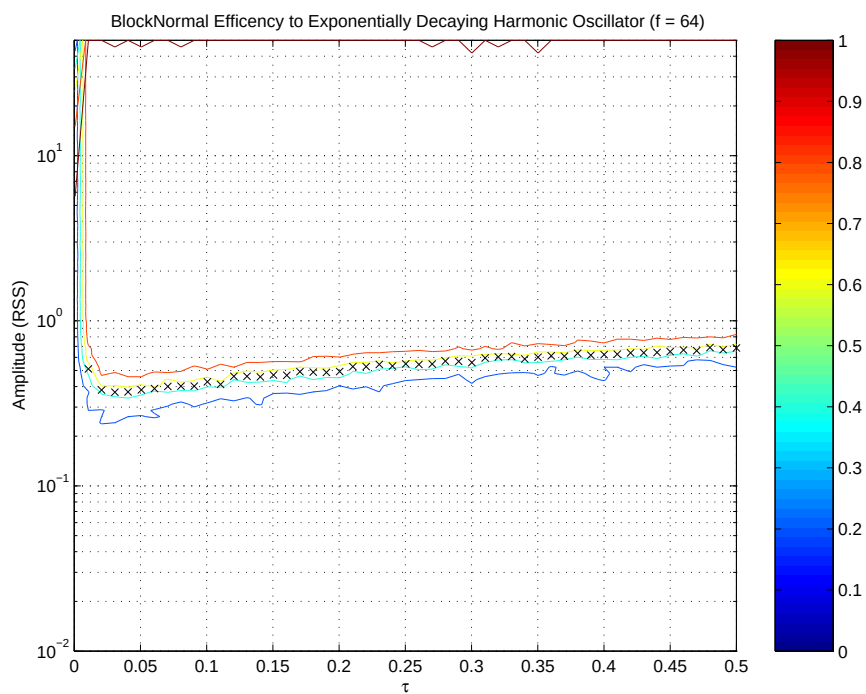
Figure F.18. BlockNormal efficiency to exponentially decaying harmonic oscillators of 64 Hz with varying amplitude and duration (shown as a contour plot) [alt tune].
