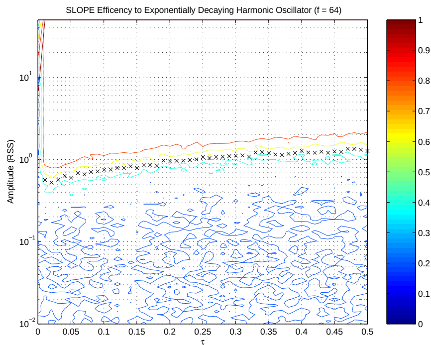
Figure F.20. SLOPE efficiency to exponentially decaying harmonic oscillators of 64 Hz with varying amplitude and duration (shown as a contour plot) [alt tune].
