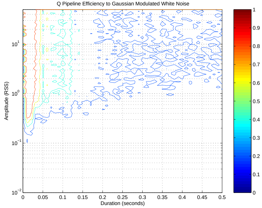
Figure 8.5. Q Pipeline efficiency to Gaussian modulated white noise with varying amplitude and duration (shown as a contour plot) [const. magnitude].
