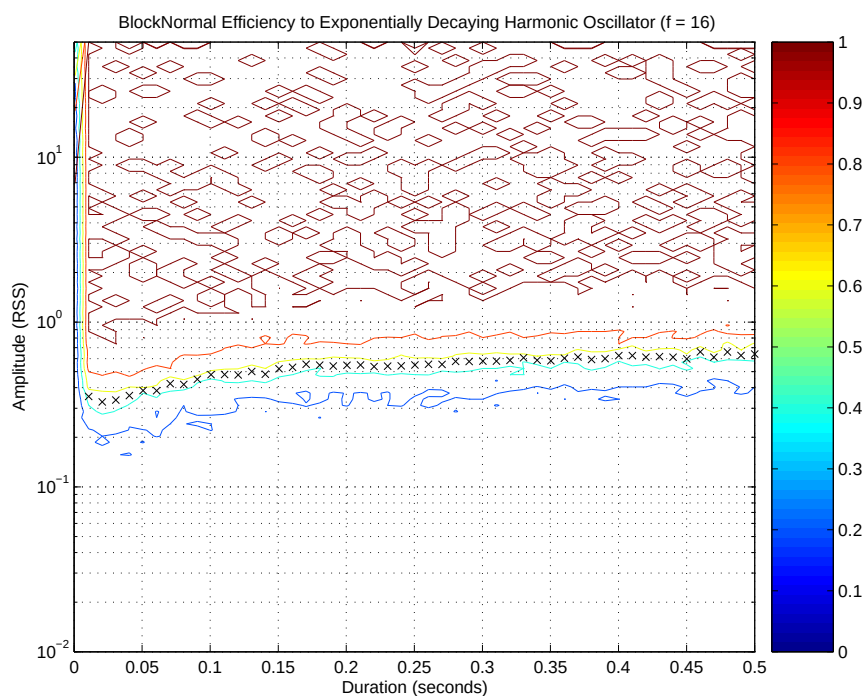
Figure E.20. BlockNormal efficiency to exponentially decaying harmonic oscillators of 16 Hz with varying amplitude and duration (shown as a contour plot).
