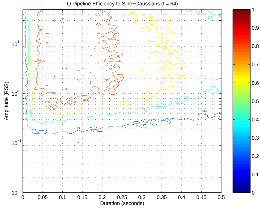
Figure 8.7. Q Pipeline efficiency to 64 Hz sine-Gaussians with varying amplitude and duration (shown as a contour plot) [const. magnitude].
