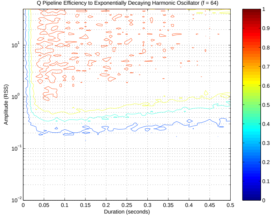
Figure 8.9. Q Pipeline efficiency to exponentially decaying harmonic oscillators of 64 Hz with varying amplitude and duration (shown as a contour plot) [const. magnitude].
