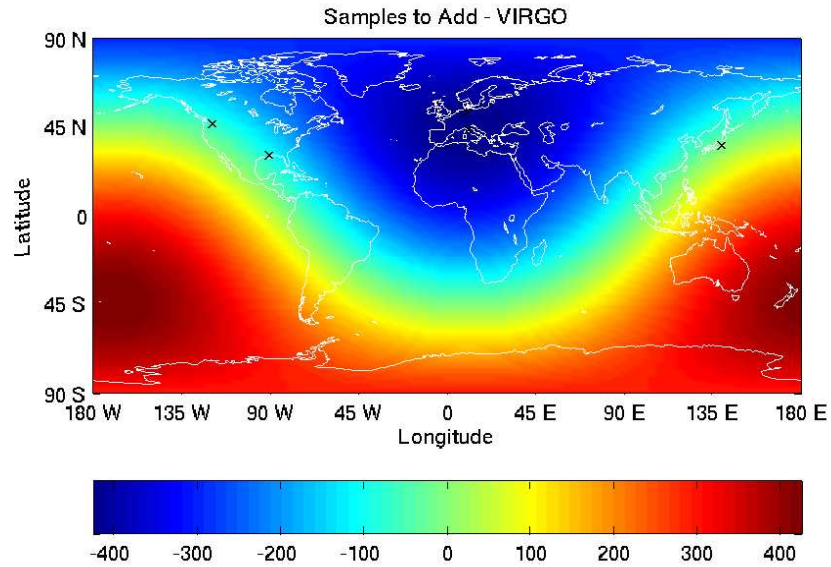
Figure A.2. The number of samples to add to signal start time with respect to the source sky location for VIRGO (sampling frequency = 20,000 samples/sec)
