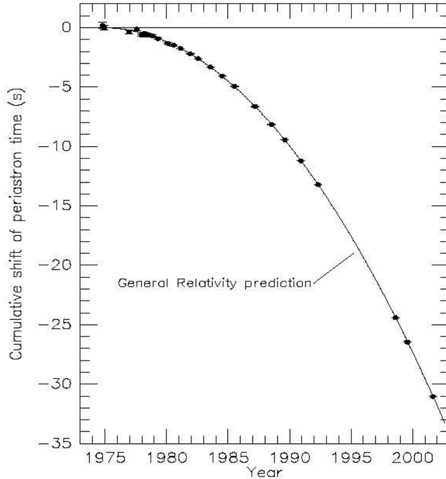
Figure 1.2. Plot of PSR 1913+16's cumulative shift in periastron since late 1974 as a function of time. The line passing through the data point's error bars represents the agreement with general relativity for the emission of energy in the form of gravitational waves. Image from [1].
