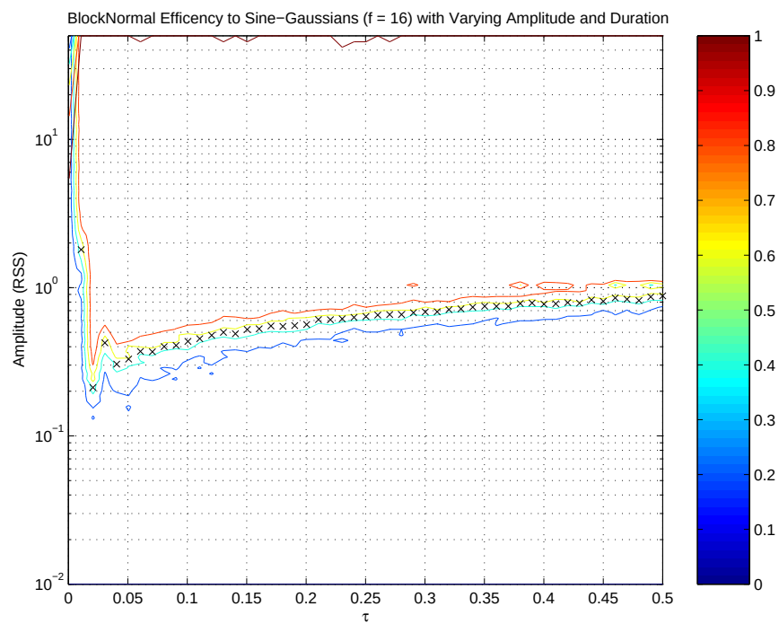
Figure F.6. BlockNormal efficiency to 16 Hz sine-Gaussians with varying amplitude and duration (shown as a contour plot) [alt tune].
