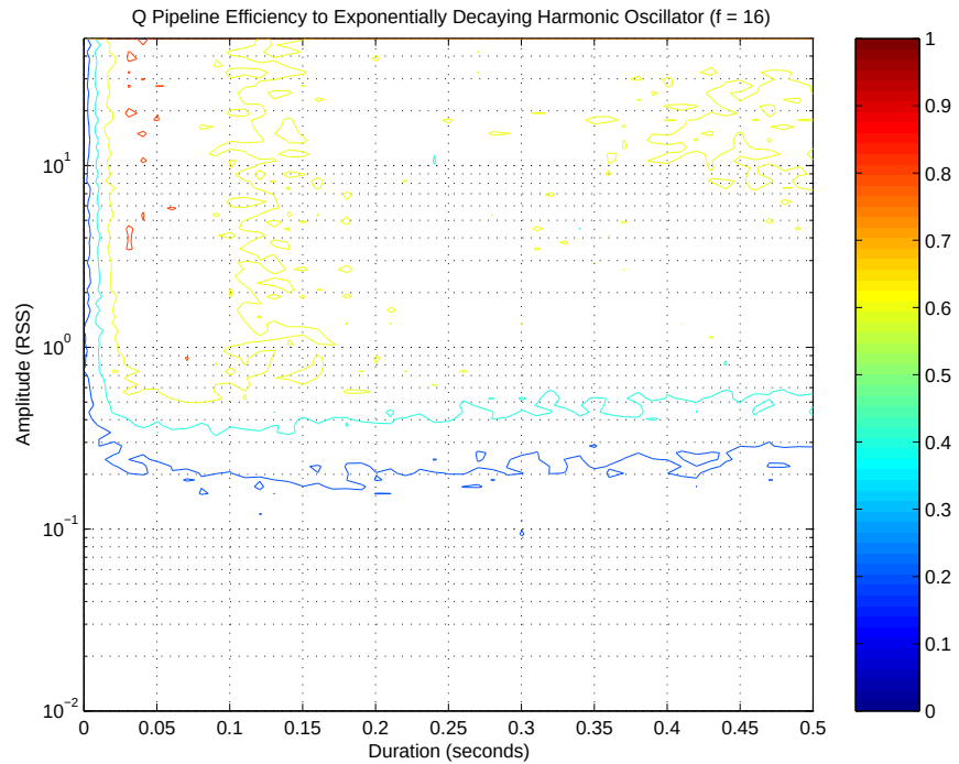
Figure 8.8. Q Pipeline efficiency to exponentially decaying harmonic oscillators of 16 Hz with varying amplitude and duration (shown as a contour plot) [const. magnitude].
