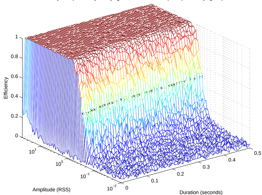
Figure E.19. BlockNormal efficiency to exponentially decaying harmonic oscillators of 16 Hz with varying amplitude and duration (shown as a 3-dimensional surface).
