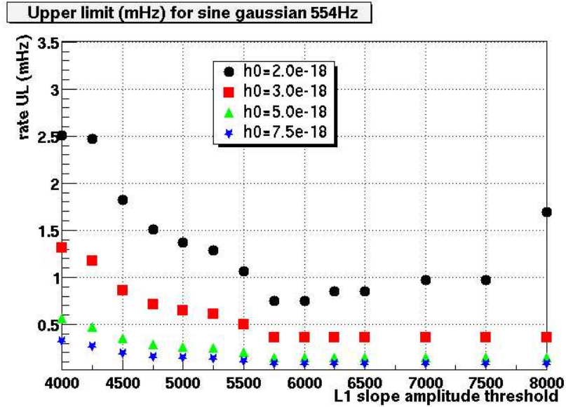
Figure 4.5. SLOPE upper limit of triple coincident triggers, with respect to threshold, for L1 with the H1 threshold held at 10,000 and the H2 threshold held at 12,800. Image courtesy of Laura Cadonati for the LIGO Burst Group [5].
