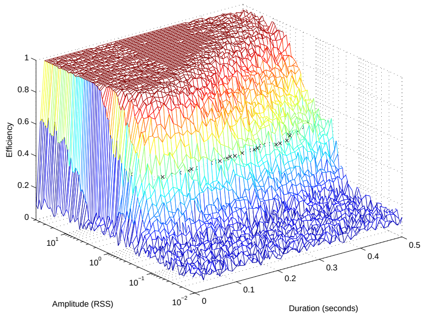
Q Pipeline Efficiency to Exponentially Decaying Harmonic Oscillator ( f = 64 ) with Varying Amplitude and Duration
