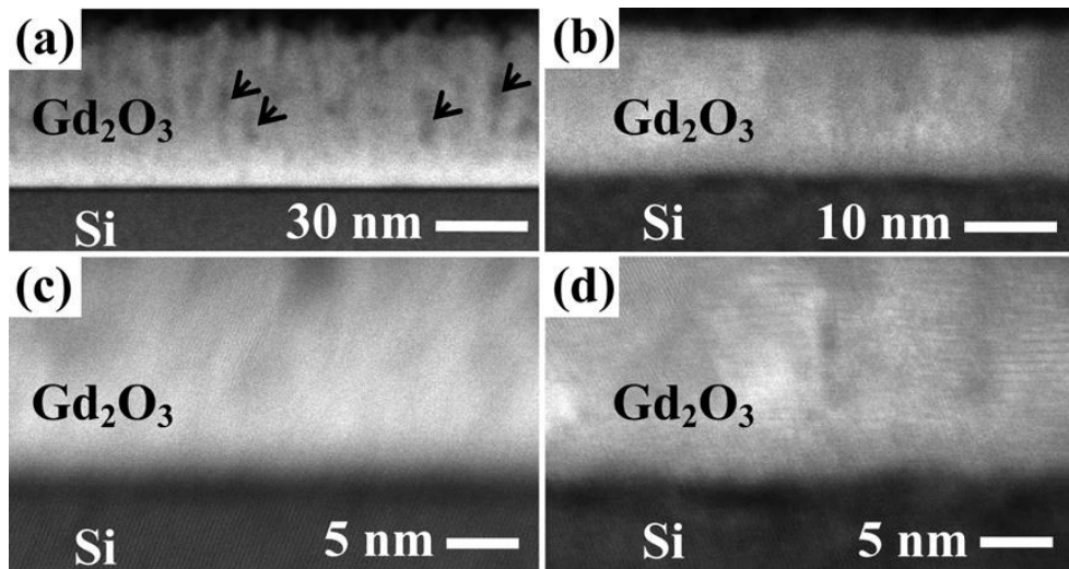
Figure 6.19. Low-magnification HAADF STEM images of thin \text{Gd}_2\text{O}_3 films (a) 8A (250 °C, 200 sccm \text{O}_2 , 47 nm) and (b) 8E (650 °C, 200 sccm \text{O}_2 , 20 nm) grown under 200 sccm oxygen flow. Higher magnification images collected near the interface regions of the (c) 8A and (d) 8E heterostructures, respectively.
