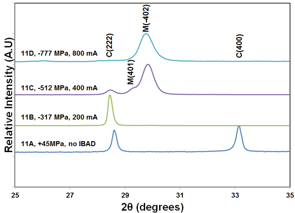
Figure 5.5. \theta - 2\theta XRD patterns of \text{Gd}_2\text{O}_3 films 11A (0 mA), 11B (200 mA), 11C (400 mA), and 11D (800 mA) grown on sapphire at 650 °C and 50 sccm \text{O}_2 under low growth rate of \sim 0.5 \text{ \AA} / \text{s} as a function of ion beam source current. 95
