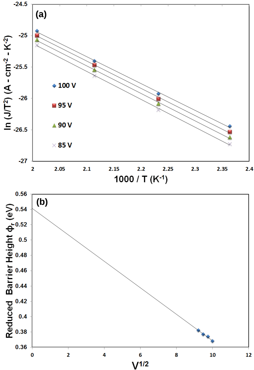
Figure 7.9. (a) Arrhenius \ln(J/T^2) vs 1/T plots used to extract reduced Schottky barrier height for various voltages (85, 90, 95, 100) and (b) extraction of effective Schottky barrier height by extrapolation of reduced barrier height vs V^{1/2} to V=0 under gate injection for film 9D (650 °C, 200 sccm O _2 , 2.69 \mu m).
