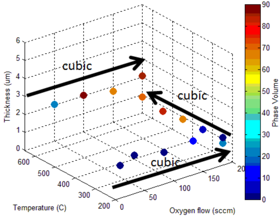
Figure 4.11. Process-phase summary map displaying the effects of temperature, oxygen flow, and thickness on the phase of \text{Gd}_2\text{O}_3 films deposited at high rates (greater than 5 \text{ \AA} / \text{s} ) by reactive electron beam physical vapor deposition (EB-PVD).
