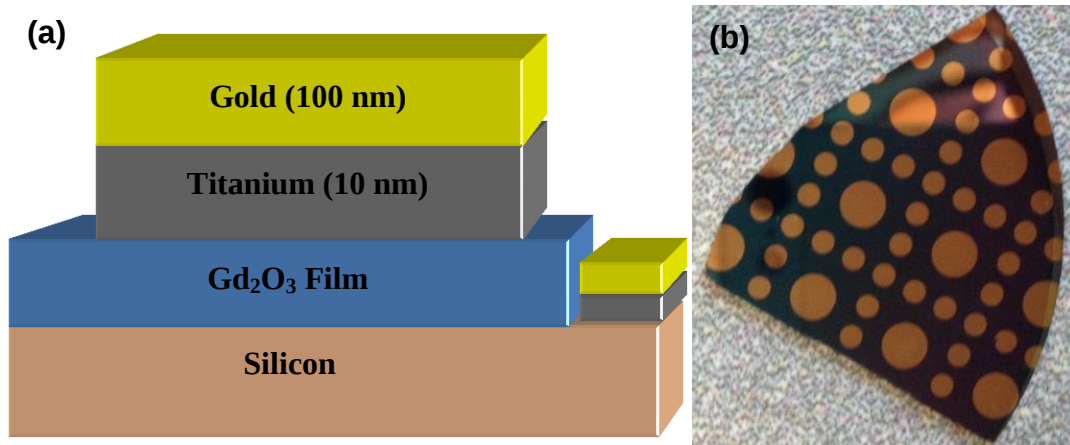
Figure 3.6. (a) Cross Sectional Schematic of Si / \text{Gd}_2\text{O}_3 / Ti / Au MOS capacitor and (b) digital image of top view of Si / \text{Gd}_2\text{O}_3 / Ti / Au MOS capacitor. The small and large circular contacts are 1.5 mm and 3 mm in diameter, respectively.
