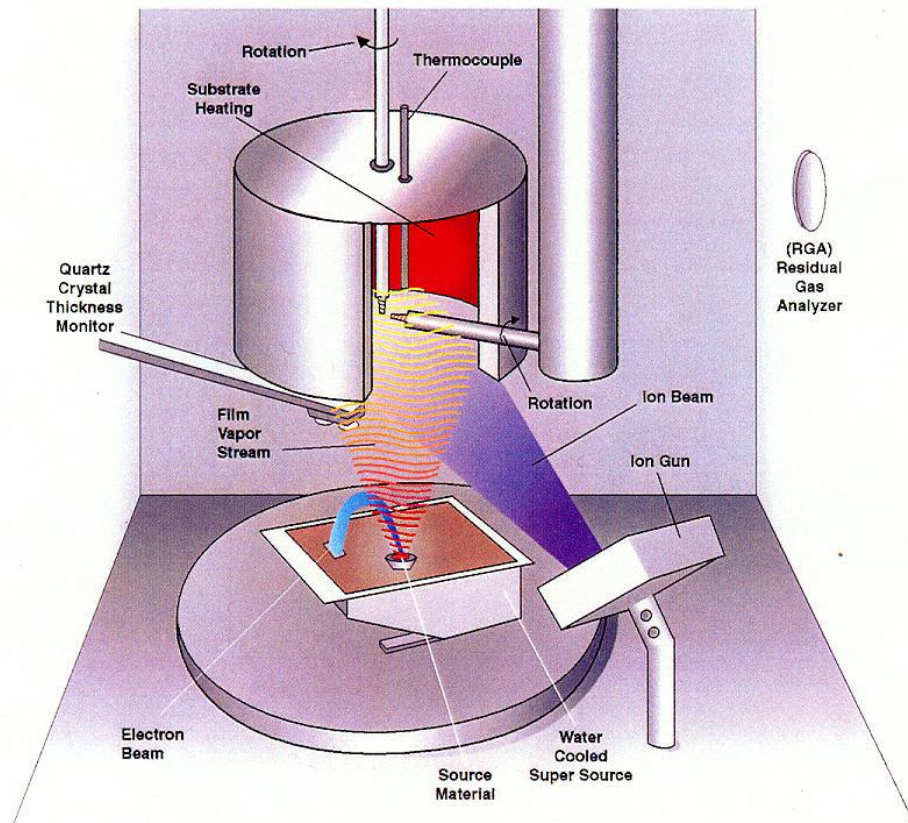
Figure 3.1. Schematic of the Denton vacuum EB-PVD system.
