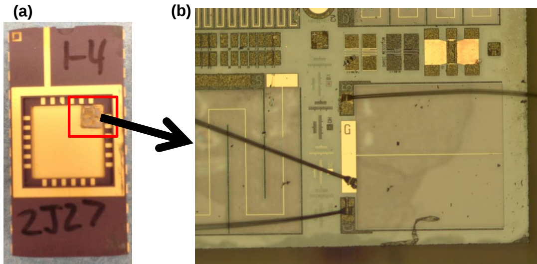
Figure 3.10. (a) Digital image of GaN / AlGaIn “rad sensor” device die attached to Cerdip packaging and (b) optical microscope image showing wirebonds to GaN / AlGaIn / \text{Gd}_2\text{O}_3 / Ti / Au MOS-HEMT terminals.
