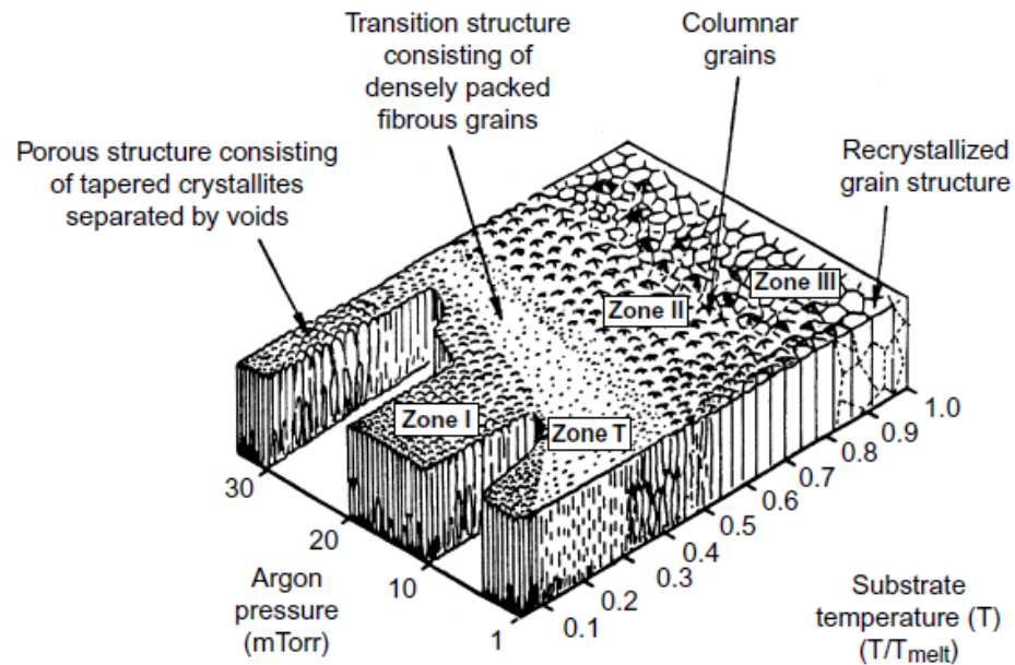
Figure 2.9. Structure-Zone model for vapor deposited coatings. The schematic contains both a top side and cross sectional view. 44
