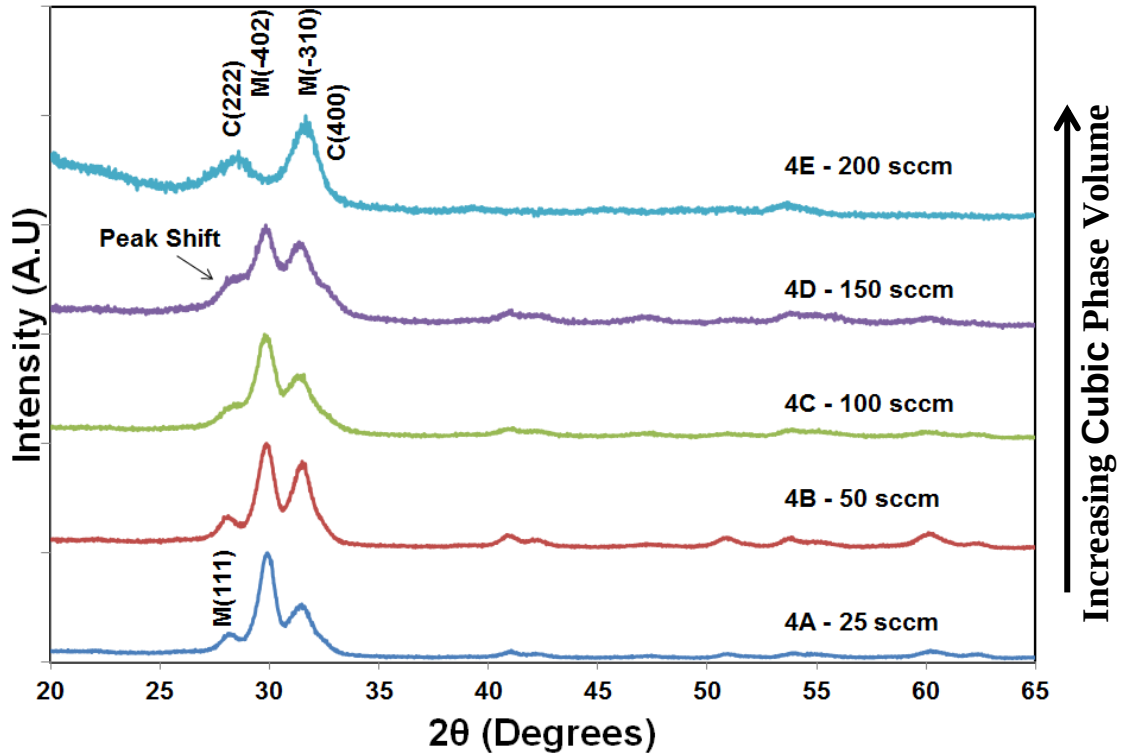
Figure 4.4. \theta -2 \theta X-ray diffraction patterns of \text{Gd}_2\text{O}_3 films 4A (25 sccm), 4B (50 sccm), 4C (100 sccm), 4D (150 sccm), and 4E (200 sccm) deposited on quartz as a function of oxygen flow at deposition temperature of 250 °C. 45
