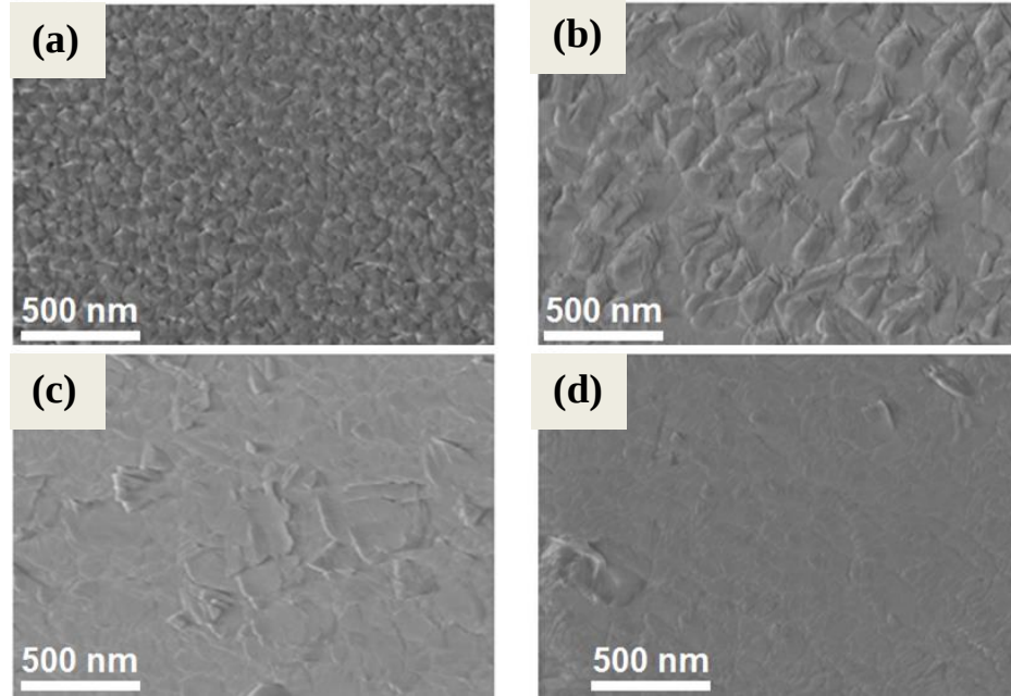
Figure 6.31. SEM top surface images of \text{Gd}_2\text{O}_3 films deposited using ion beam assisted deposition with currents of (a) 11A (0 mA), (b) 11B (200 mA), (c) 11C (400 mA), and (d) 11D (800 mA) deposited on sapphire as a function of IBS current at 650 °C, 50 sccm \text{O}_2 , and with growth rate of \sim 0.5 \text{ \AA} / \text{s} .
