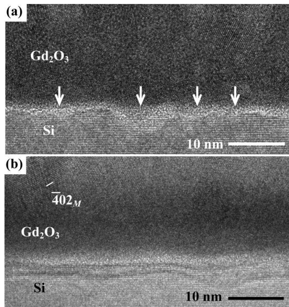
Figure 6.17. High-resolution TEM images collected from the interfacial regions of \text{Gd}_2\text{O}_3 films (a) 6A (250 °C, 200 sccm \text{O}_2 , 1.07 \mu\text{m} ) and (b) 6E (650 °C, 200 sccm \text{O}_2 , 0.87 \mu\text{m} ) deposited on silicon under 200 sccm \text{O}_2 at high rates ( > 5 \text{ \AA} / \text{s} ).
