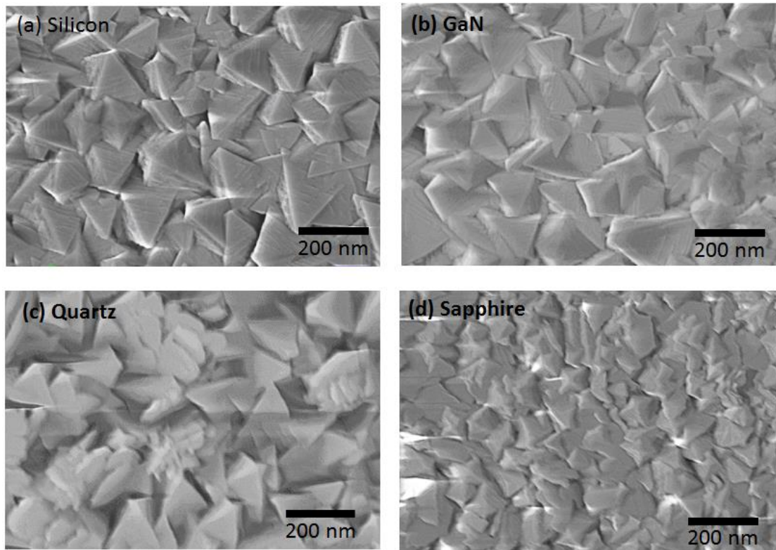
Figure 6.25. SEM surface images of Gd 2 O 3 film 10A (650 °C, 50 sccm O 2 , 1.01 \mu m, 0.5 Å / s) on (a) silicon(111), (b) GaN, (c) quartz, and (d) sapphire substrates.
