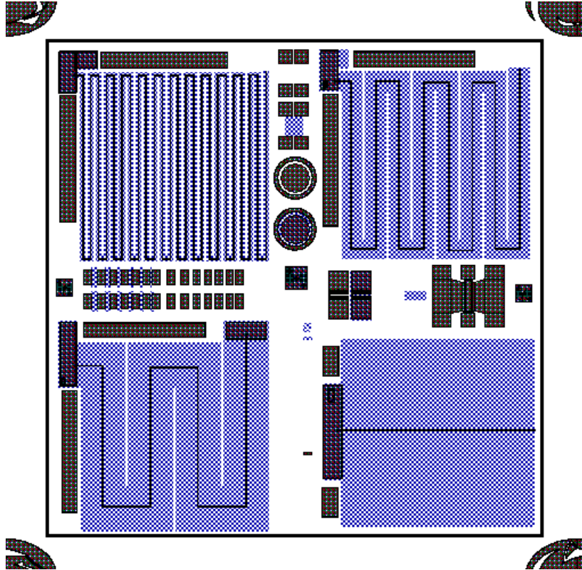
Figure A.5. Schottky level mask layout for GaN / AlGaIn rad sensor device fabrication.
