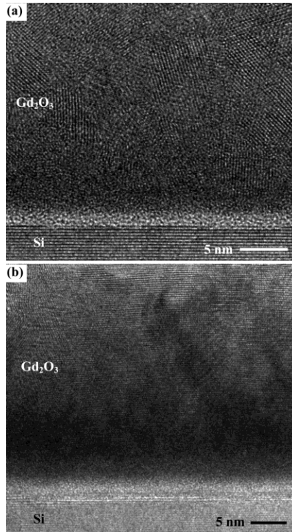
Figure 6.18. High-resolution TEM images collected from the interfacial regions of \text{Gd}_2\text{O}_3 films (a) 7A (250 °C, 50 sccm \text{O}_2 , 1.11 \mu\text{m} ) and (b) 7E (650 °C, 50 sccm \text{O}_2 , 1.20 \mu\text{m} ) deposited on silicon under 50 sccm \text{O}_2 at high rates ( > 5 \text{ \AA} / \text{s} ).
