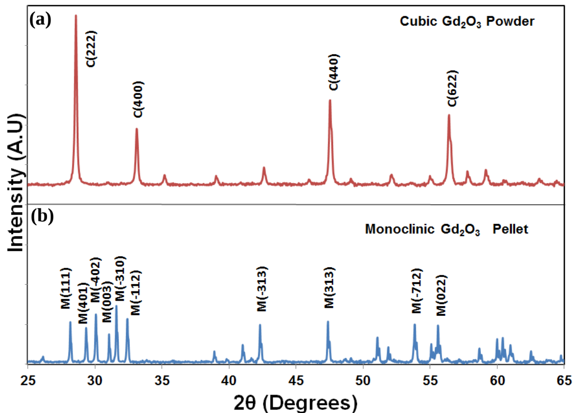
Figure 4.2. \theta - 2\theta X-ray diffraction patterns of (a) fully cubic \text{Gd}_2\text{O}_3 powder and (b) fully monoclinic \text{Gd}_2\text{O}_3 pellet after sintering at 1400 °C used to estimate the difference in diffracted intensity between the two phases.
