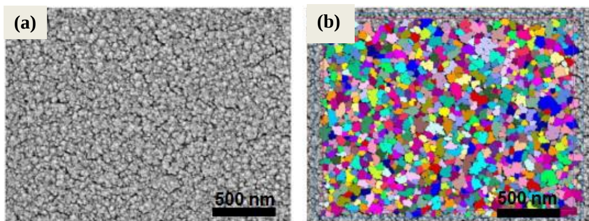
Figure 6.5. (a) SEM surface image of film 2A ( 250^\circ\text{C} , 200 sccm \text{O}_2 , 1.26\ \mu\text{m} ) and (b) the corresponding grain size measurement technique. The measured grain size was 51.2 \pm 1.6\ \text{nm} for film 2A deposited at 250^\circ\text{C} under 200 sccm \text{O}_2 flow.
