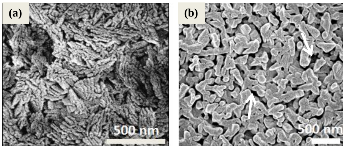
Figure 6.33. SEM top surface images of mixed phase film 12E (650 °C, 200 sccm \text{O}_2 , 1.2 \mu\text{m} ) in the following conditions: (a) as deposited and (b) heat treated at 1000 °C in \text{O}_2 environment for 1 hour. Arrows denote porous regions.
