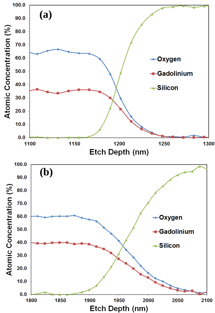
Figure 6.38. Atomic composition of Gd 2 O 3 films (a) 2A (250°C, 200 sccm O 2 , 1.26 μm) and (b) 2E (650°C, 200 sccm O 2 , 2.05 μm) as a function of etch depth.
