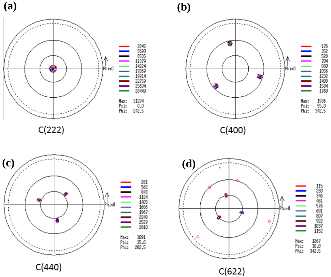
Figure 5.14. Pole figures of (a) C(222), (b) C(400), (c) C(440), and (d) C(622) planes for film 11B (650 °C, 50 sccm \text{O}_2 , 0.5 Å / s, 200 mA) deposited on sapphire using ion beam assisted deposition (IBAD) showing very strong in and out-of-plane texture.
