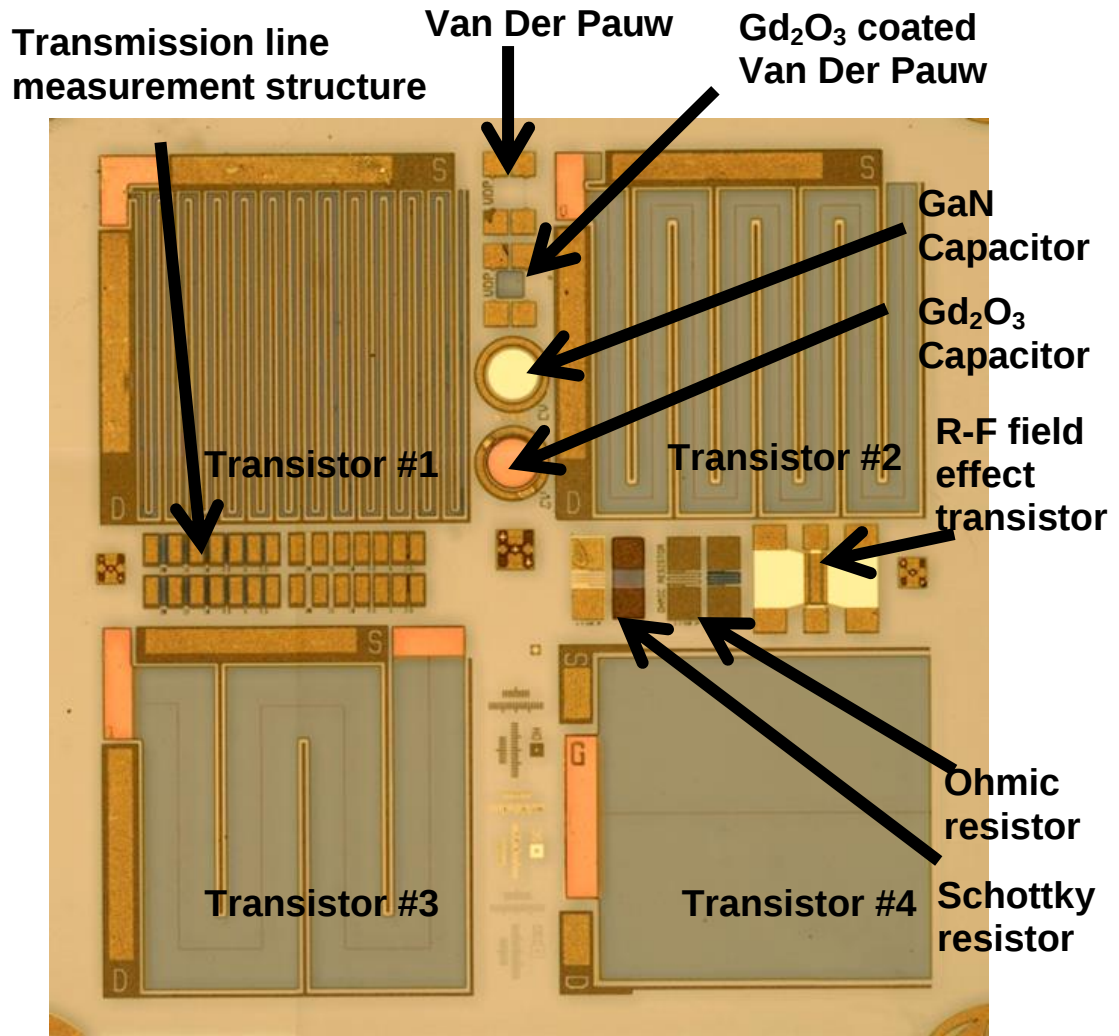
Figure 3.8. Optical microscope image of top surface of GaN / AlGaN based “rad sensor” structures. The device contains a number of electrical test structures including four high electron mobility transistors (HEMTs) with different device geometries, transmission line measurement structures, Van Der Pauw structures, MOS capacitors, an RF-Field effect transistor, an ohmic resistor, and a Schottky resistor. The labels S, D, and G correspond to the source, drain, and gate for each of the four transistor structures.
