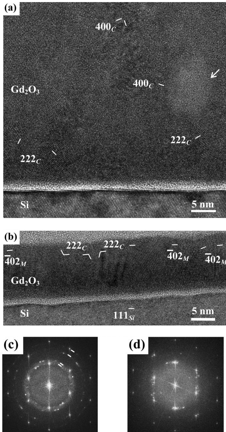
Figure 6.3. High-resolution TEM images of thin \text{Gd}_2\text{O}_3 films (a) 8A (250 °C, 200 sccm \text{O}_2 , 47 nm) and (b) 8E (650 °C, 200 sccm \text{O}_2 , 20 nm). A few crystallographic planes were indicated by short white lines and labeled. FFT patterns of (c) 8A and (d) 8E. Four spotty rings are marked by short white lines in (c). 105
