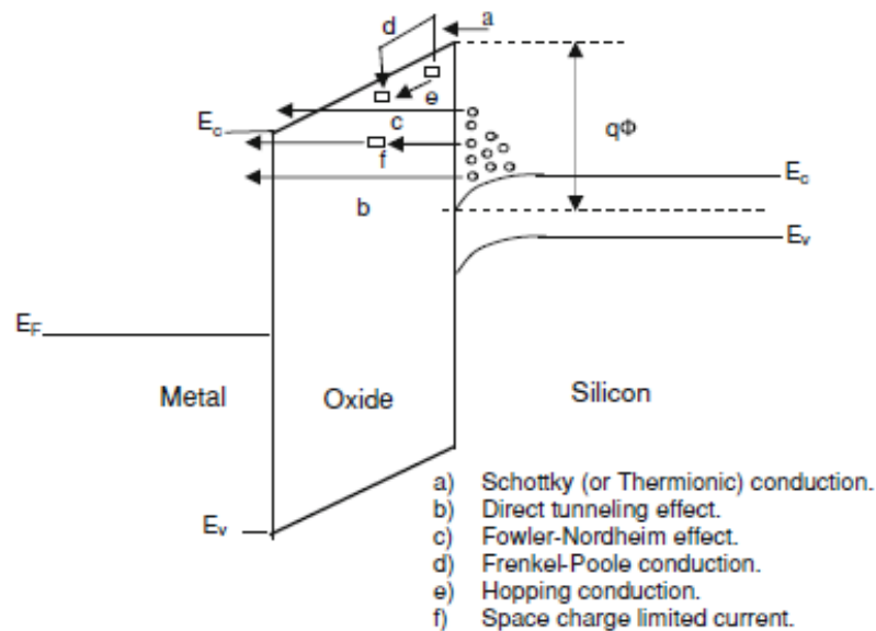
Figure 2.13. Energy level transitions for different conduction mechanisms. E_v is the valence band, E_c is the conduction band, E_f is the Fermi level, and q\Phi is the Schottky barrier height. 66
