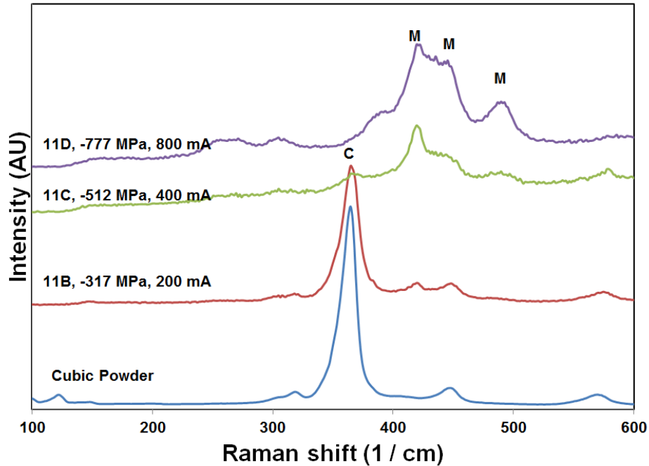
Figure 5.6. Raman spectra of cubic \text{Gd}_2\text{O}_3 powder and \text{Gd}_2\text{O}_3 films 11B (200 mA), 11C (400 mA), and 11D (800 mA) grown on sapphire at 650\text{ }^\circ\text{C} and 50 sccm \text{O}_2 under low growth rate of \sim 0.5\text{ \AA/s} as a function of ion source current.
