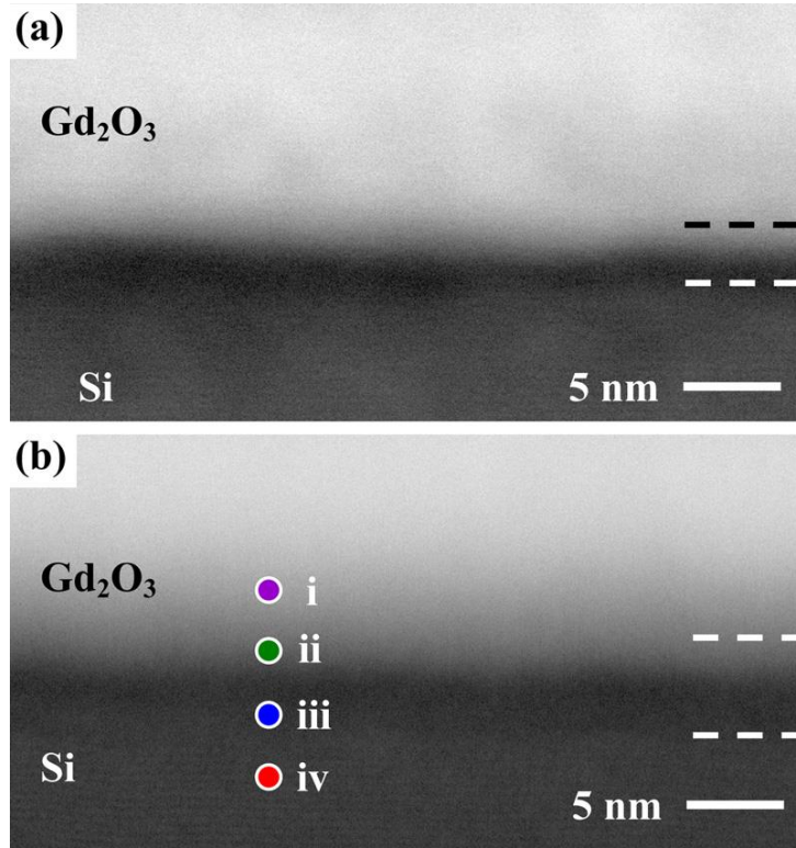
Figure 6.23. HAADF STEM images collected from the interfacial region of the thick \text{Gd}_2\text{O}_3 films at (a) 7A (250 °C, 50 sccm \text{O}_2 , 1.11 \mu\text{m} ) and (b) 7E (650 °C, 50 sccm \text{O}_2 , 1.20 \mu\text{m} ) grown under 50 sccm oxygen. The top and bottom dashed lines indicate the approximate positions of the \text{Gd}_2\text{O}_3 /interfacial layer and interfacial layer/Si boundaries, respectively.
