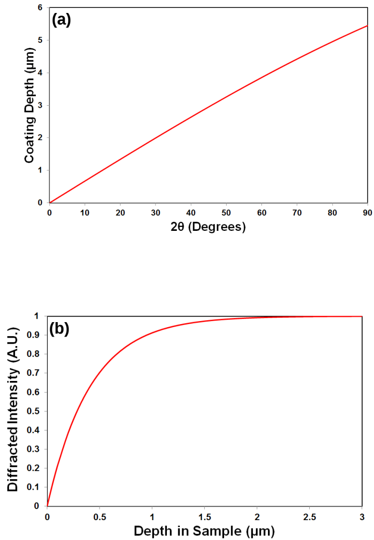
Figure 3.4. (a) \text{Gd}_2\text{O}_3 film thickness from which 99% of the intensity originates as a function of angle 2\theta and (b) percentage of diffracted intensity as a function of \text{Gd}_2\text{O}_3 film thickness at the Si(111) peak position.
