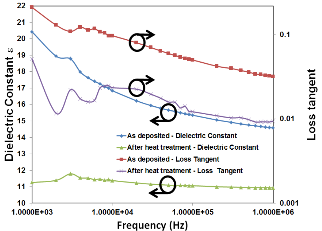
Figure 7.1. Dispersion of the dielectric constant and loss tangent of a \text{Gd}_2\text{O}_3 film as a function of frequency (a) as deposited and (b) after heat treatment at 100 °C. Arrows denote corresponding y axis.
