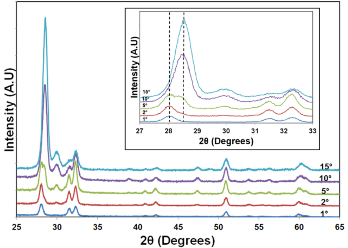
Figure 4.6. Grazing incidence diffraction patterns taken at incident angles of 1, 2, 5, 10, and 15 ° for film 6E (650 °C, 200 sccm O 2 , 0.87 \mu m) deposited on quartz. The inset shows the magnified M(111) and C(222) peaks located at 28.0 and 28.6 °, respectively.
