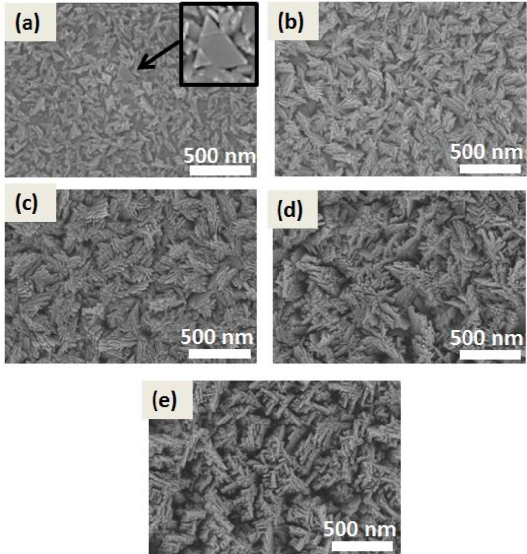
Figure 6.15. SEM morphology of \text{Gd}_2\text{O}_3 films (a) 9A (0.38 \mu\text{m} ), (b) 9B (0.59 \mu\text{m} ), (c) 9C (1.02 \mu\text{m} ), and (d) 9D (2.69 \mu\text{m} ), and (e) 9E (5.72 \mu\text{m} ) deposited on Si(111) at 650 ^\circ\text{C} under 200 sccm \text{O}_2 flow at high rates ( > 5 \text{ \AA} / \text{s} ). The inset in Figure 6.15a shows a C(222) triangular facet.
