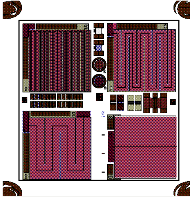
Figure A.1. Overall mask layout for GaN / AlGaN rad sensor device fabrication.
