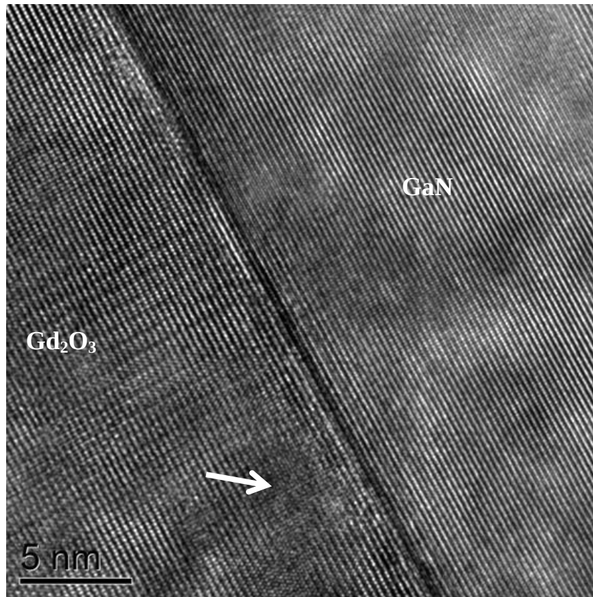
Figure 6.29. (a) High-resolution TEM image collected from the interfacial region of \text{Gd}_2\text{O}_3 film 10A (650 °C, 50 sccm \text{O}_2 , 1.01 \mu\text{m} , 0.5 \text{\AA} / s) deposited on GaN. The arrow denotes a defect region.
