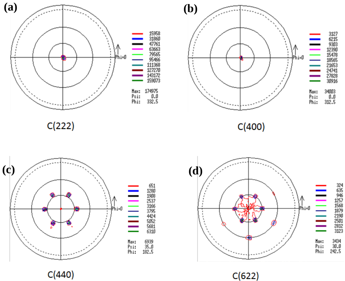
Figure 5.12. Pole figures of (a) C(222), (b) C(400), (c) C(440), and (d) C(622) planes for film 10B (650 °C, 50 sccm O 2 , 0.5 Å / s) deposited on GaN showing strong in and out-of-plane texture.
