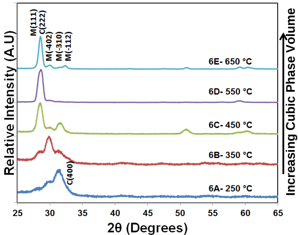
Figure 4.1. \theta - 2\theta X-ray diffraction patterns of \text{Gd}_2\text{O}_3 films 6A ( 250^\circ\text{C} ), 6B ( 350^\circ\text{C} ), 6C ( 450^\circ\text{C} ), 6D ( 550^\circ\text{C} ), and 6E ( 650^\circ\text{C} ) deposited on quartz as a function of temperature under 200 sccm \text{O}_2 flow.
