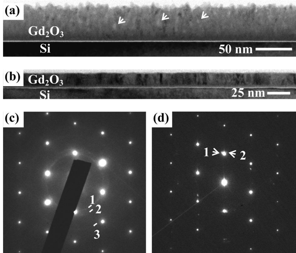
Figure 6.2. Low-magnification bright-field TEM images of thin \text{Gd}_2\text{O}_3 films (a) 8A (250 °C, 200 sccm \text{O}_2 , 47 nm) and (b) 8E (650 °C, 200 sccm \text{O}_2 , 20 nm). The arrows denote porous regions. The corresponding SAD patterns are shown in (c) and (d), respectively.
