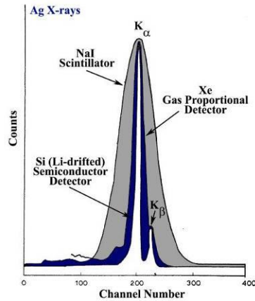
Figure 2.1. Energy spectrum of detectors illustrating superior energy resolution of the semiconductor-based detection method. 1
