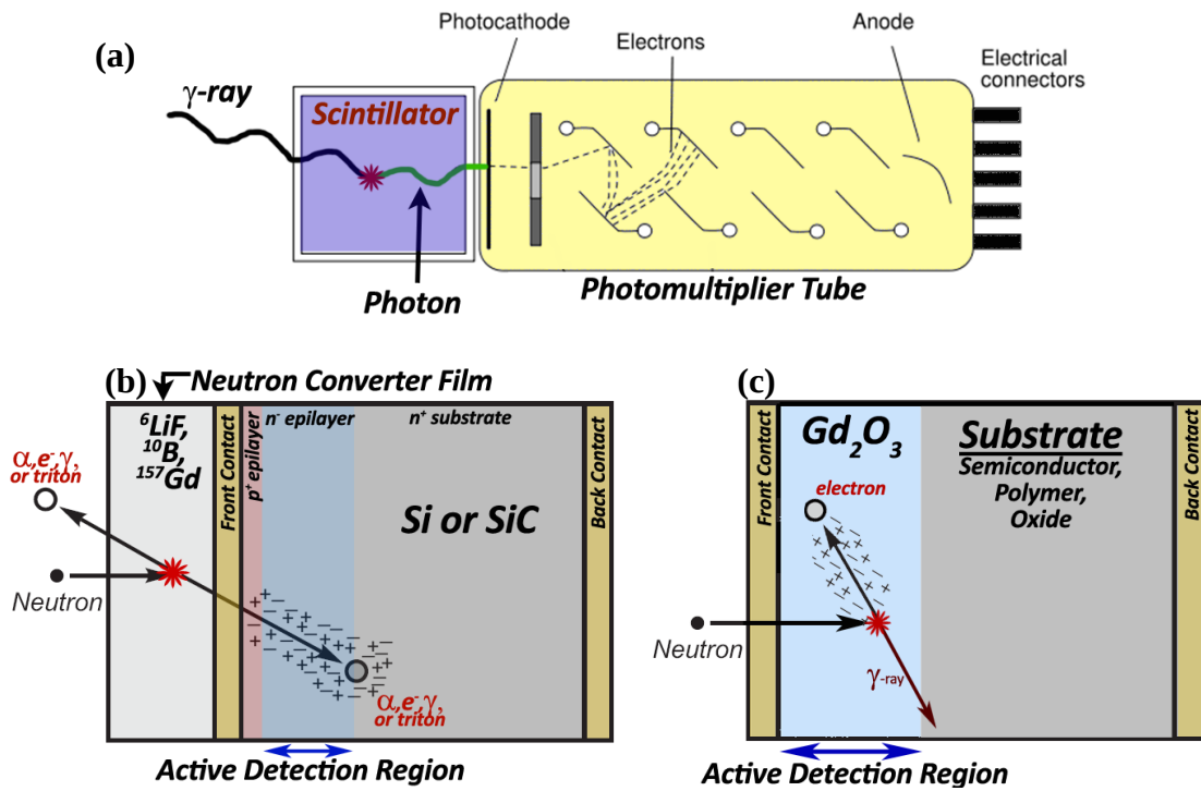
Figure 2.3. Schematic representations of (a) scintillator solid state detector, (b) silicon-based state-of-the-art solid state detector, and (c) Gd 2 O 3 solid state device.
