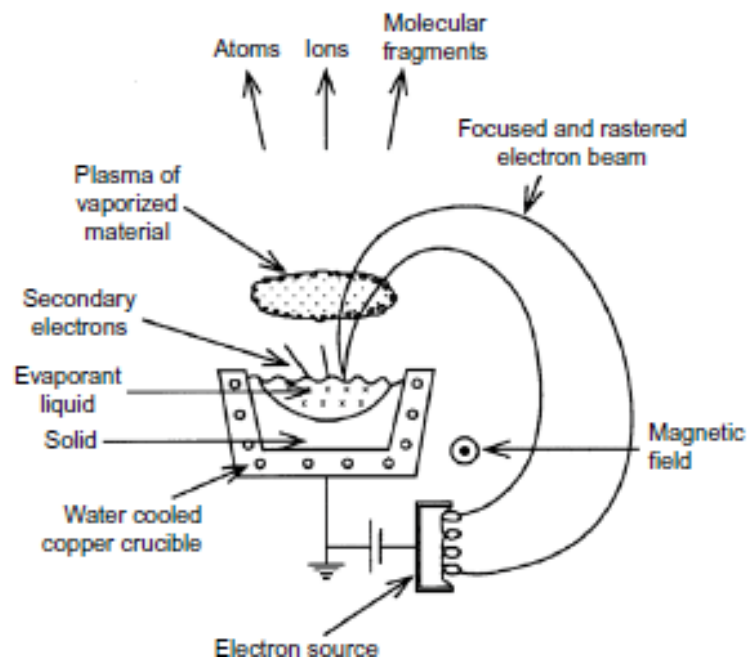
Figure 2.7. Schematic of electron beam-physical vapor deposition process. 40
