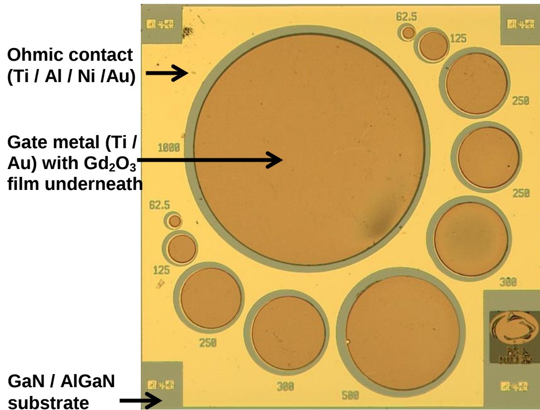
Figure 3.7. Optical microscope image of GaN / AlGaIn based “dot-ring” structure with several MOS capacitors with diameters ranging from 62.5 \mu\text{m} to 1 mm.
