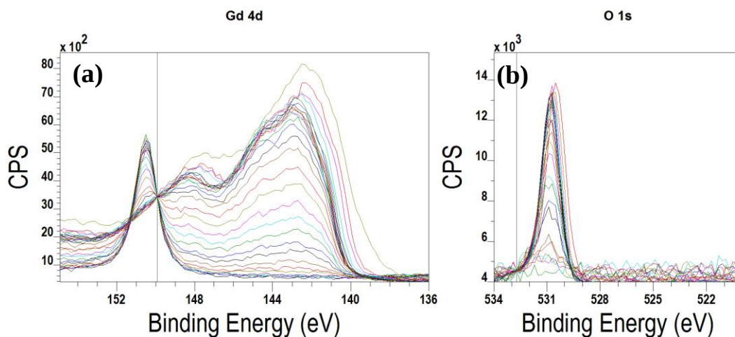
Figure 6.36. Depth profile of XPS binding energy levels of (a) Gd 4d and (b) O1s of film 2E (650 °C, 200 sccm O 2 , 2.05 µm).
