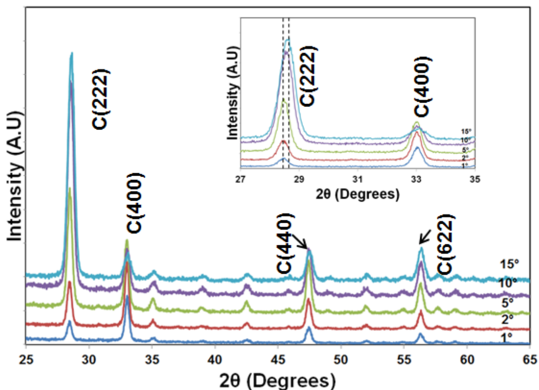
Figure 5.7. Grazing incidence diffraction patterns taken at incidence angles of 1, 2, 5, 10, and 15 degrees for film 10B (650 °C, 50 sccm \text{O}_2 , 910 nm, 0.5 Å/s) deposited on quartz. The inset shows the magnified C(222) and C(400) peaks.
