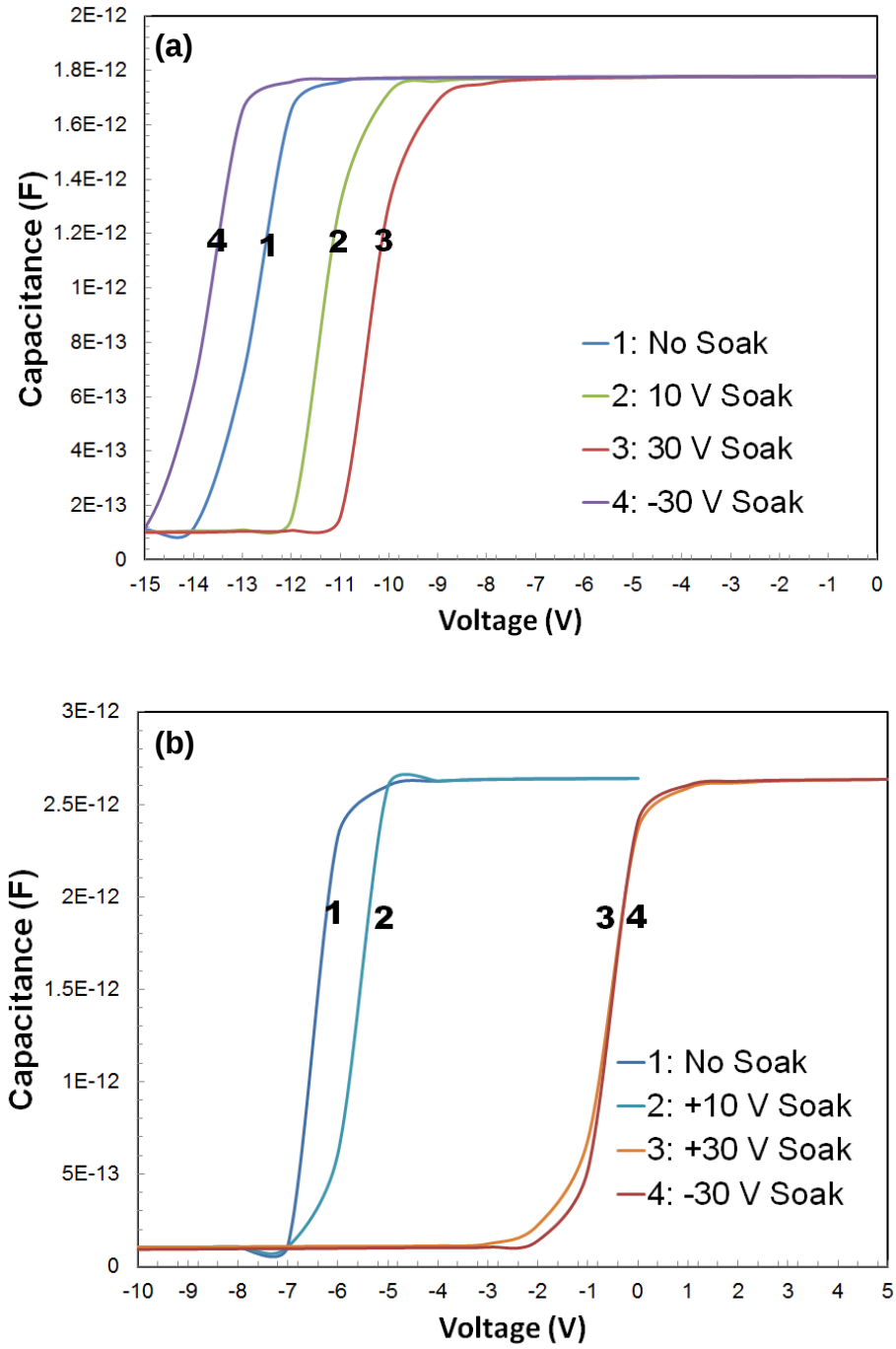
Figure 7.5. C-V curves for GaN / AlGaIn / Gd 2 O 3 / Ti / Au MOS capacitors (a) 6A (250 °C, 200 sccm O 2 , 1.07 μm) and (b) 10A (650 °C, 50 sccm O 2 , 1.01 μm, 0.5 Å/s).
