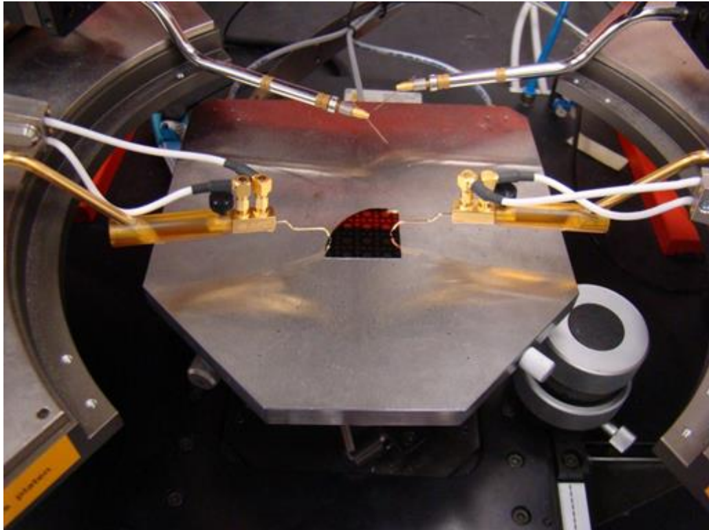
Figure 3.9. Capacitance-voltage (C-V) measurement of Si(111) / \text{Gd}_2\text{O}_3 / Ti / Au MOS capacitor using a Suss PM5 probe station with probes connected to Keithley 4200 Semiconductor Characterization System.
