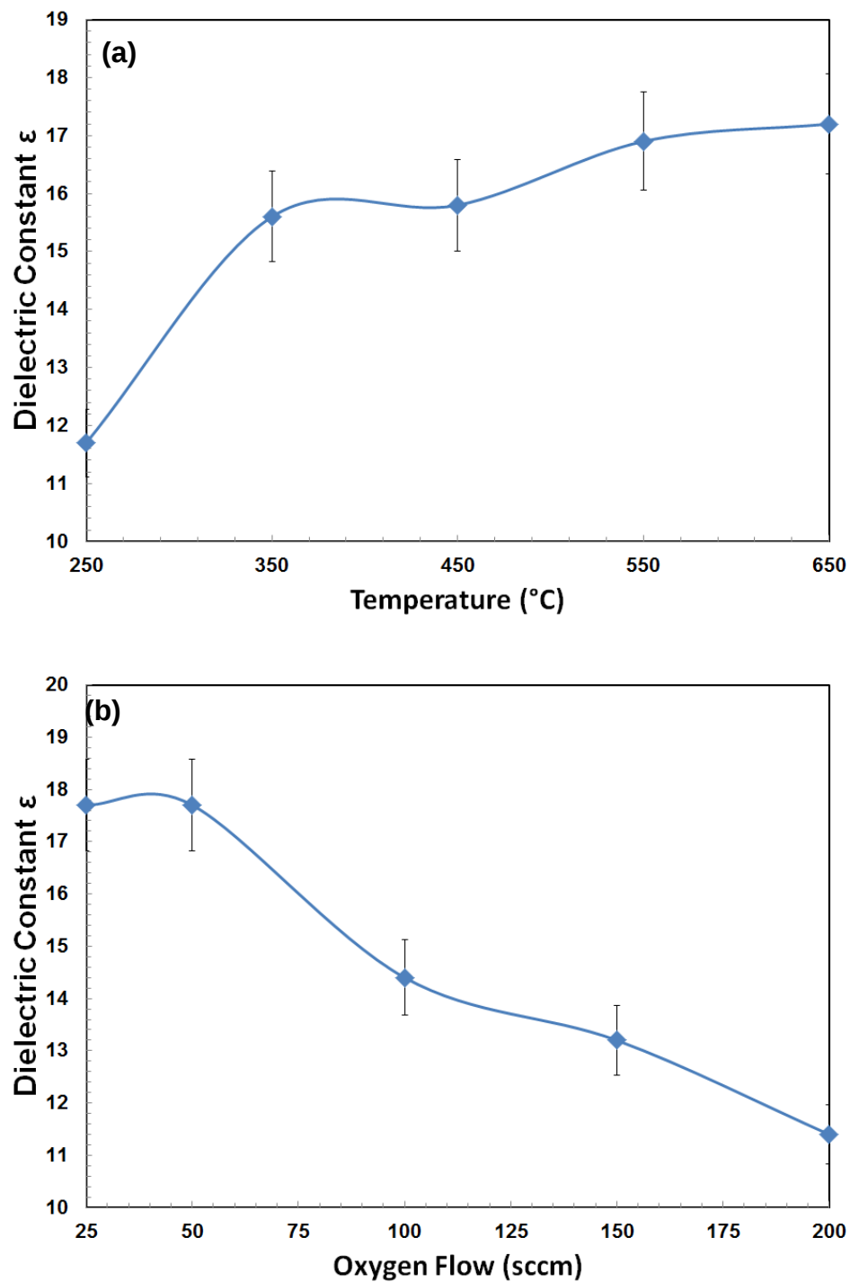
Figure 7.2. \text{Gd}_2\text{O}_3 permittivity measured at a frequency of 1 MHz as a function of (a) temperature of films 6A-6E (function of temperature, 200 sccm \text{O}_2 , \sim 1 \mu\text{m} ) and (b) oxygen flow rate for films 4A-4E (250 °C, function of \text{O}_2 flow, \sim 1 \mu\text{m} ).
