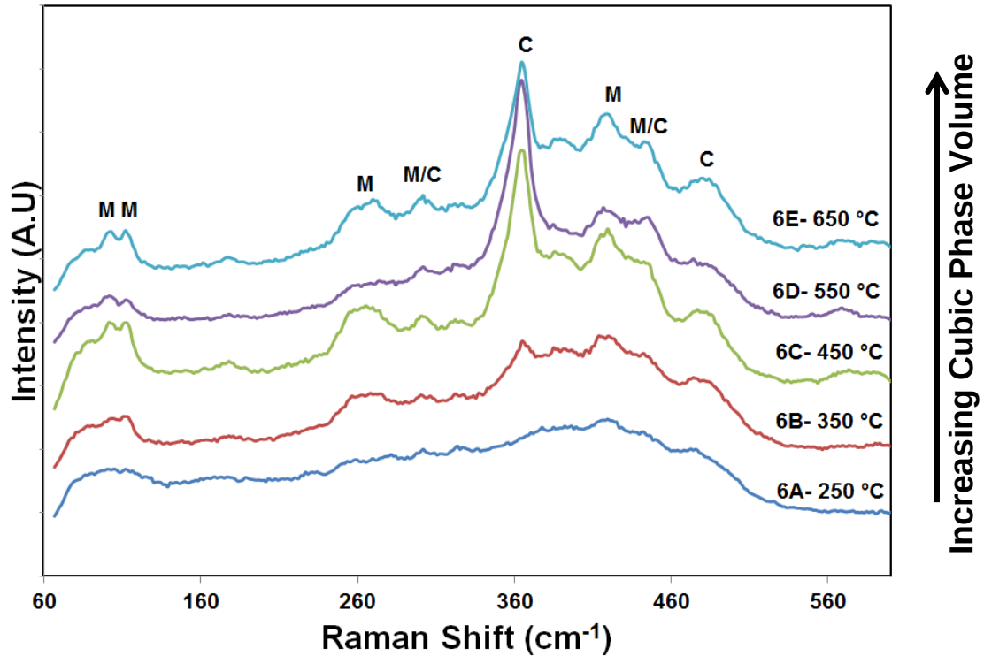
Figure 4.3. Raman spectra of Gd 2 O 3 films 6A (250 °C), 6B (350 °C), 6C (450 °C), 6D (550 °C), and 6E (650 °C) deposited on quartz as a function of temperature under 200 sccm O 2 flow. The cubic and monoclinic bands used for quantitative phase volume analysis are marked C and M, respectively.
