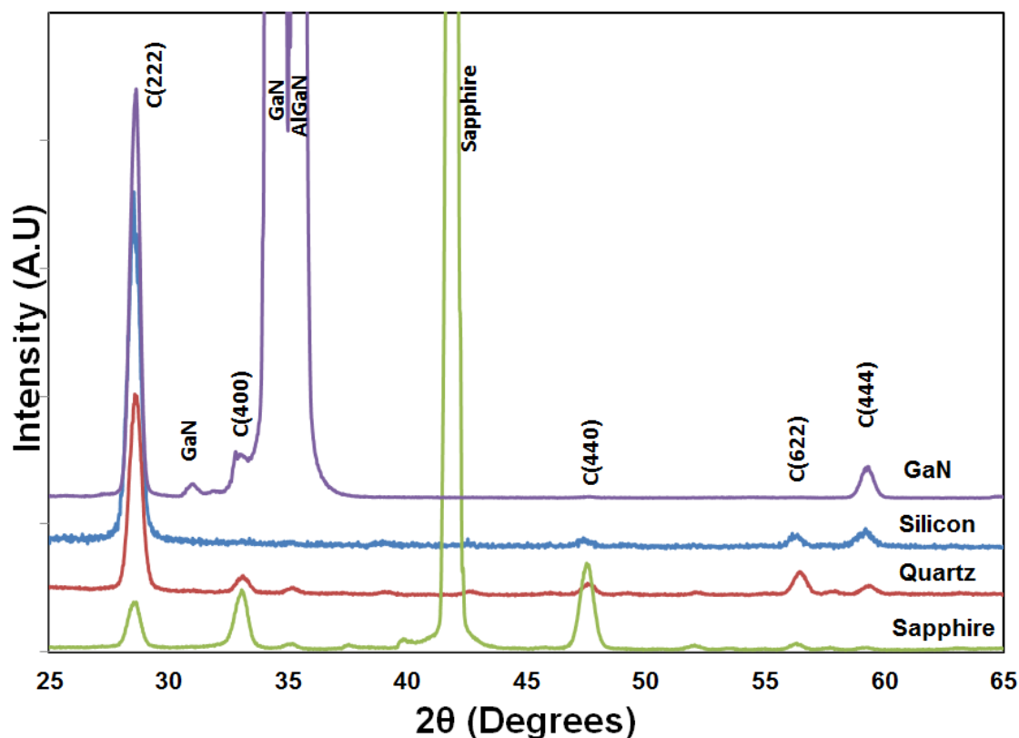
Figure 5.4. 0-2 \theta X-ray diffraction patterns of fully cubic Gd 2 O 3 film 10B (650 °C, 50 sccm O 2 , 910 nm, 0.5 Å/s) deposited on sapphire, quartz, silicon, and GaN.
