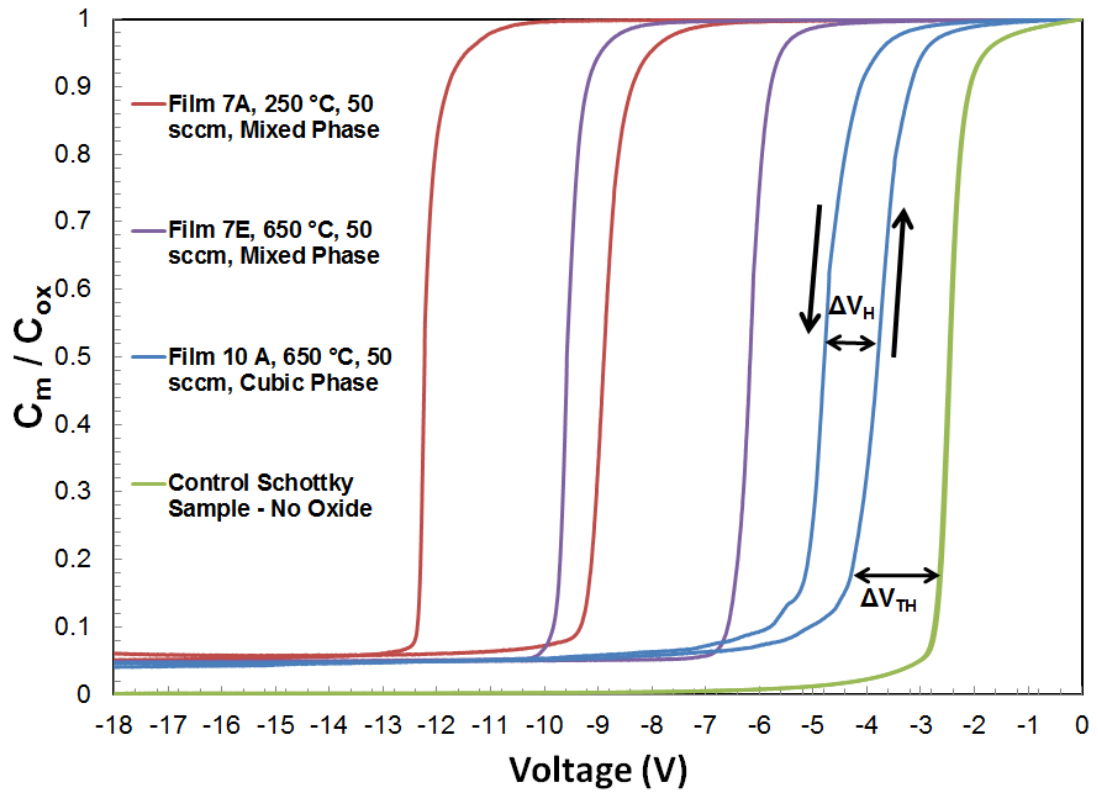
Figure 7.3. Capacitance-Voltage curves taken at 1 MHz for GaN / AlGaIn / \text{Gd}_2\text{O}_3 / Ti / Au MOS capacitors 7A (250 °C, 50 sccm \text{O}_2 , 1.1 \mu\text{m} ), 7E (650 °C, 50 sccm \text{O}_2 , 1.20 \mu\text{m} ), 10A (650 °C, 50 sccm \text{O}_2 , 1.01 \mu\text{m} , 0.5 \text{\AA} /s) and GaN / AlGaIn / Ti / Au Schottky control sample.
