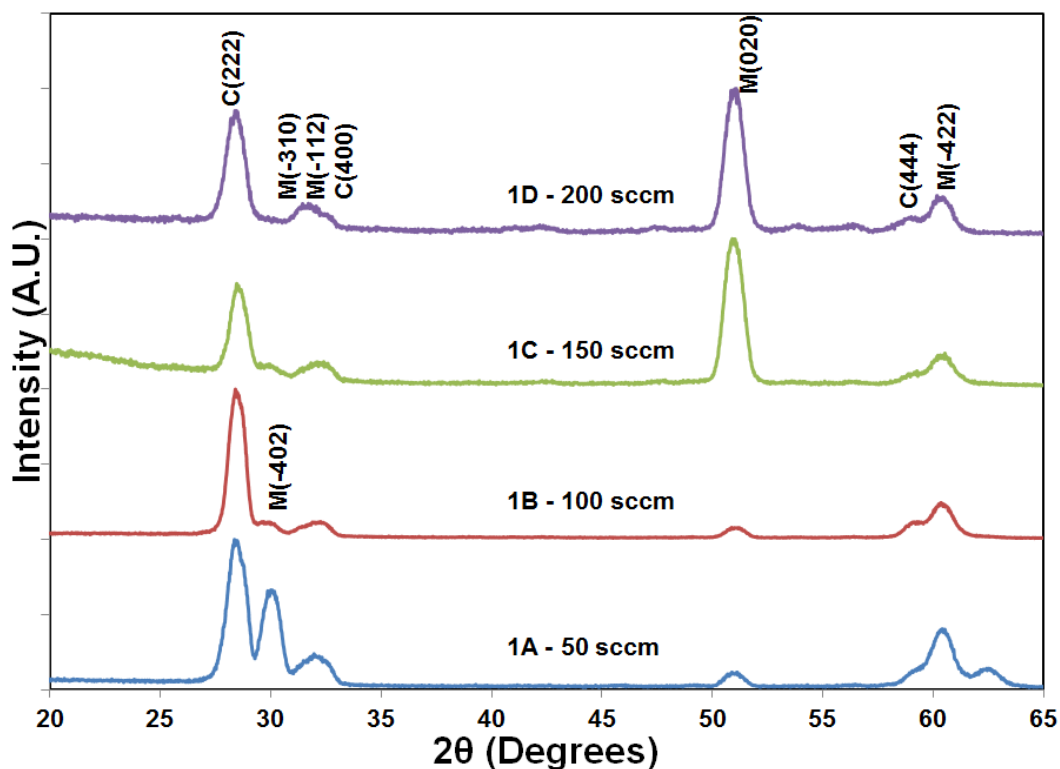
Figure 4.5. \theta -2 \theta X-ray diffraction patterns of \text{Gd}_2\text{O}_3 films 1A (50 sccm \text{O}_2 ), 1B (100 sccm \text{O}_2 ), 1C (150 sccm \text{O}_2 ), and 1D (200 sccm \text{O}_2 ) deposited on quartz as a function of oxygen flow at a deposition temperature of 650 ^\circ\text{C} .
