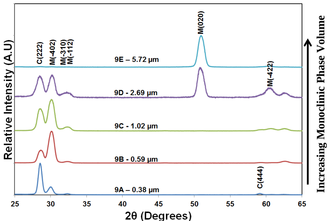
Figure 4.8. \theta -2 \theta X-ray diffraction patterns of \text{Gd}_2\text{O}_3 films 9A (0.38 \mu\text{m} ), 9B (0.59 \mu\text{m} ), 9C (1.02 \mu\text{m} ), 9D (2.69 \mu\text{m} ), and 9E (5.72 \mu\text{m} ) deposited on quartz as a function of thickness at deposition temperature of 650 ^\circ\text{C} and under 200 sccm of \text{O}_2 flow.
