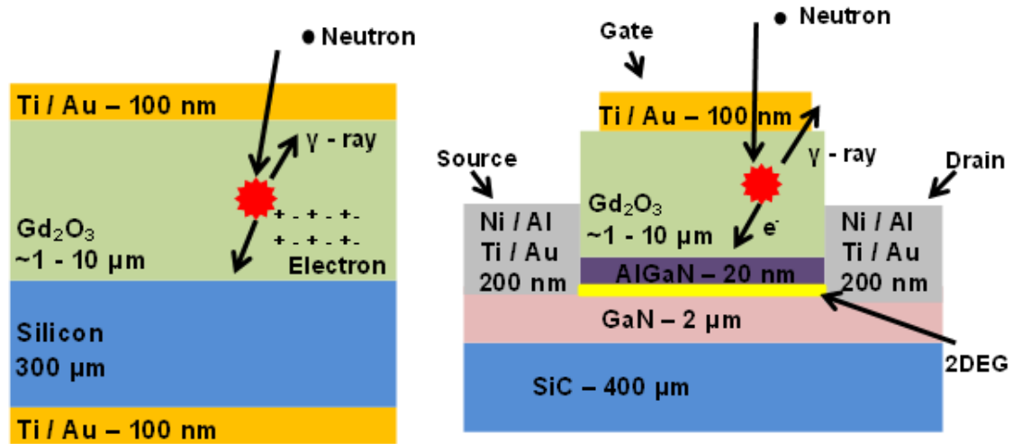
Figure 1.1. Schematic showing radiation test structures based on (a) silicon-based electronics and (b) AlGaIn/GaN based electronics. Figures not drawn to scale.
