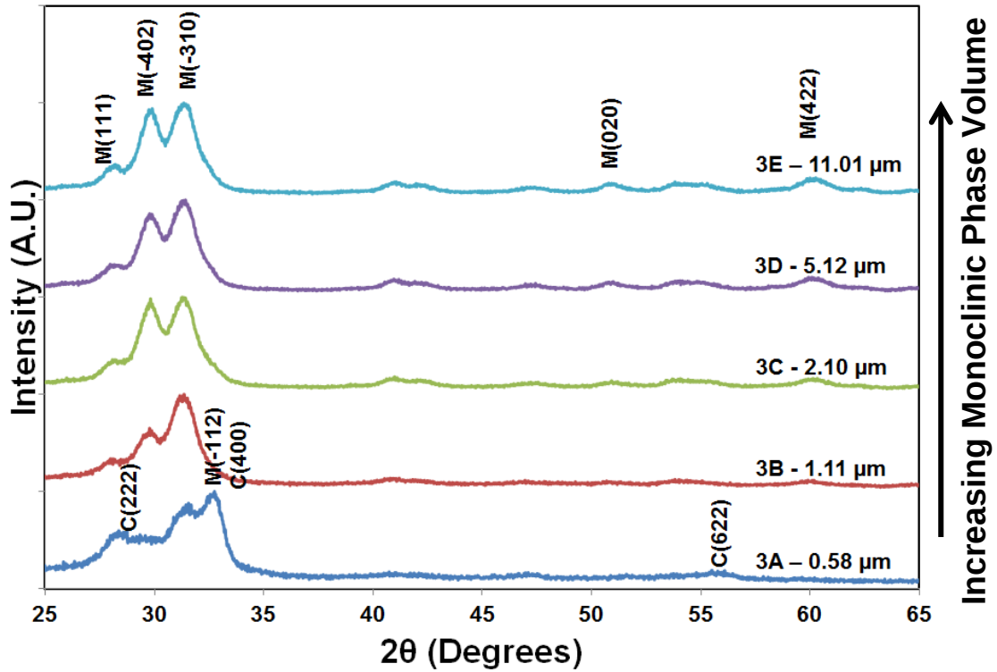
Figure 4.7. \theta -2 \theta X-ray diffraction patterns of \text{Gd}_2\text{O}_3 films 3A (0.58 \mu\text{m} ), 3B (1.11 \mu\text{m} ), 3C (2.10 \mu\text{m} ), 3D (5.12 \mu\text{m} ), and 3E (11.01 \mu\text{m} ) deposited on quartz as a function of film thickness at deposition temperature of 250 ^\circ\text{C} and oxygen flow rate of 200 sccm.
