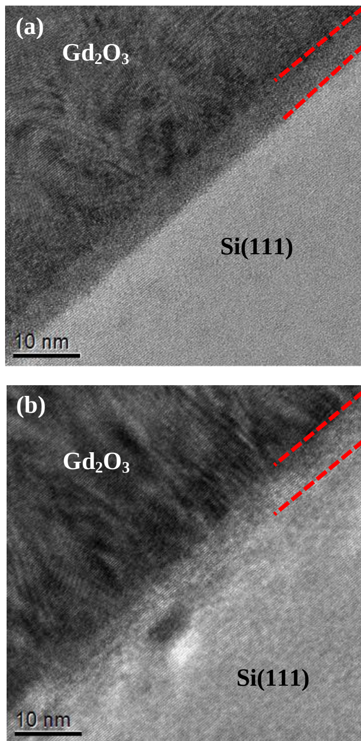
Figure 6.27. High-resolution TEM images collected from the interfacial region of the \text{Gd}_2\text{O}_3 film 10A (650 °C, 50 sccm \text{O}_2 , 1.01 \mu\text{m} , 0.5 \text{\AA}/\text{s} ) deposited on silicon showing (a) amorphous and (b) crystalline character. The dashed lines denote the interfacial region.
