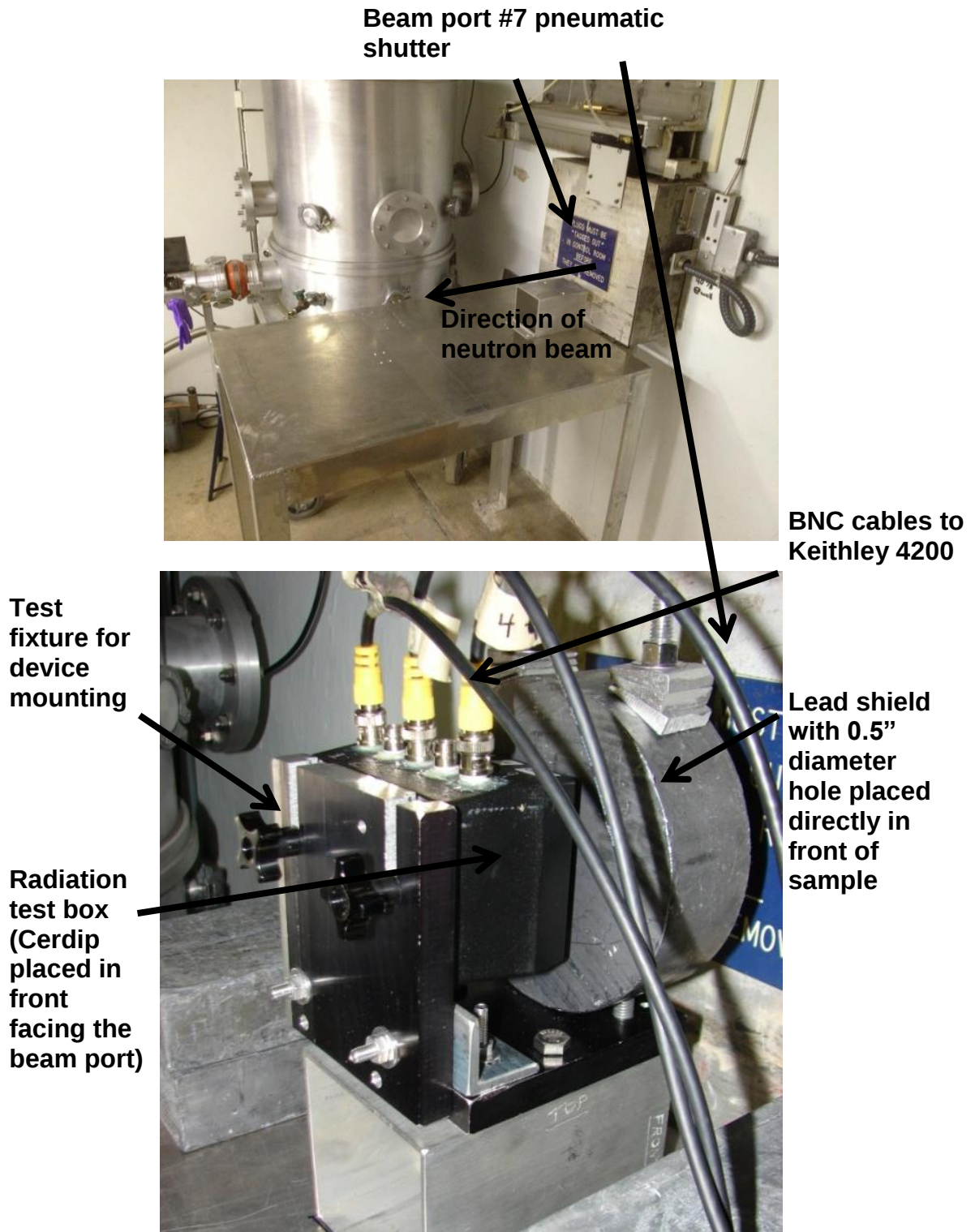
Figure 3.11. Digital images of (a) beam lab housing beam port #7 and (b) radiation detector fixture with lead shield and cable connections to electronics.
