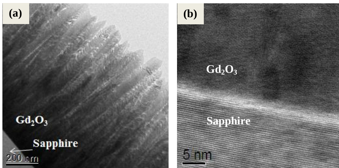
Figure 6.30. (a) Low-magnification and (b) high-magnification bright-field TEM images of \text{Gd}_2\text{O}_3 film 10A (650 °C, 50 sccm \text{O}_2 , 1.01 \mu\text{m} , 0.5 \text{\AA} / s) deposited on sapphire.
