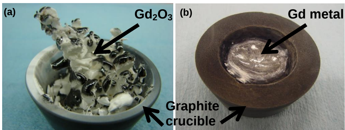
Figure 3.3. Digital images of (a) \text{Gd}_2\text{O}_3 and (b) Gd source material after direct and reactive evaporations, respectively.
