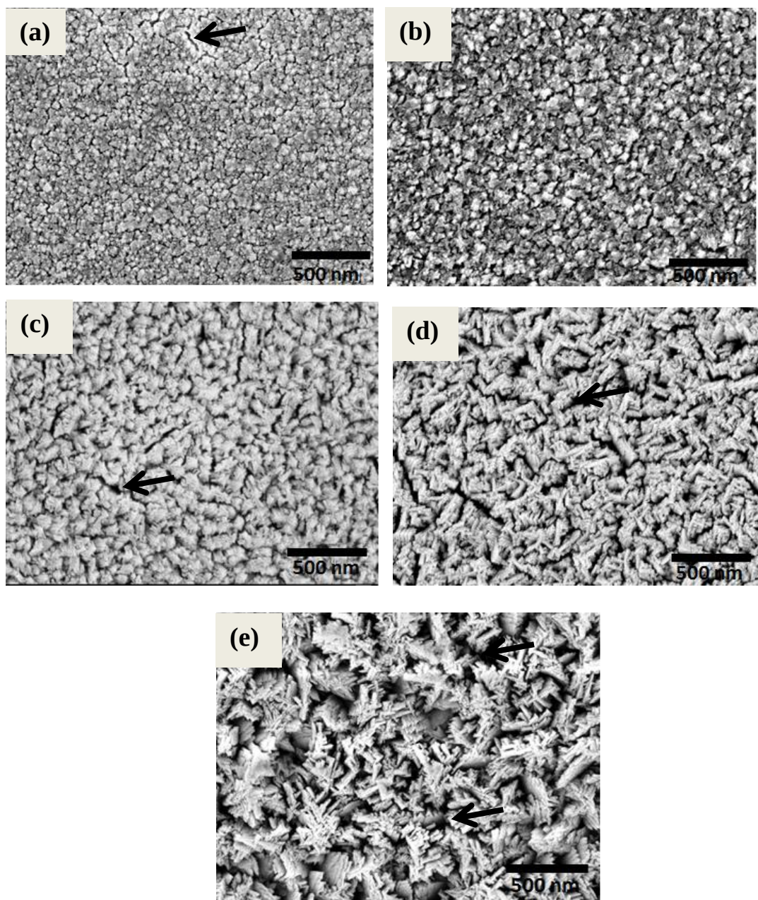
Figure 6.4. SEM top surface images of \text{Gd}_2\text{O}_3 films (a) 2A (250 °C), (b) 2B (350 °C), (c) 2C (450 °C), (d) 2D (550 °C), and (e) 2E (650 °C) deposited as a function of temperature under 200 sccm \text{O}_2 flow at high rates ( > 5 \text{ \AA} / \text{s} ). Arrows denote voiding.
