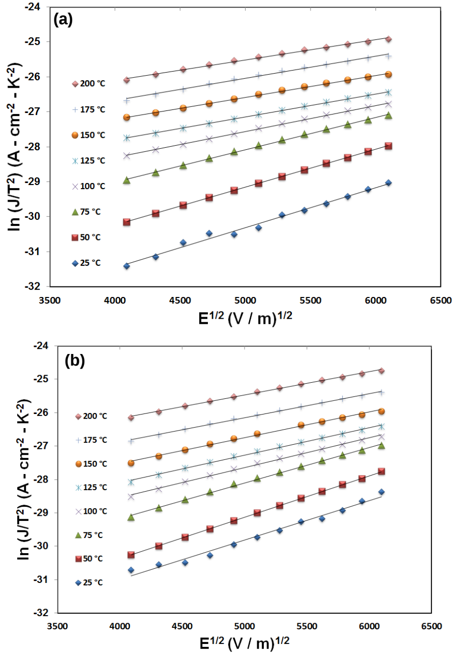
Figure 7.8. Schottky emission plots ( \ln(J/T^2) vs E^{1/2} ) under (a) gate injection and (b) substrate injection for Gd 2 O 3 film 9D (650 °C, 200 sccm O 2 , 2.69 \mu m).
