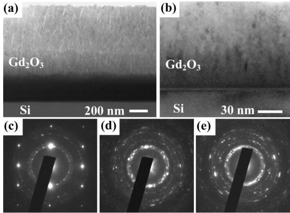
Figure 6.10. (a) Low-magnification and (b) high-magnification bright-field TEM images of thick Gd_2O_3 film 7A (250 °C, 50 sccm O_2 , 1.11 \mu m ). SAD patterns collected from the (c) interfacial region, (d) the middle section, and (e) the top section of the film, respectively.
