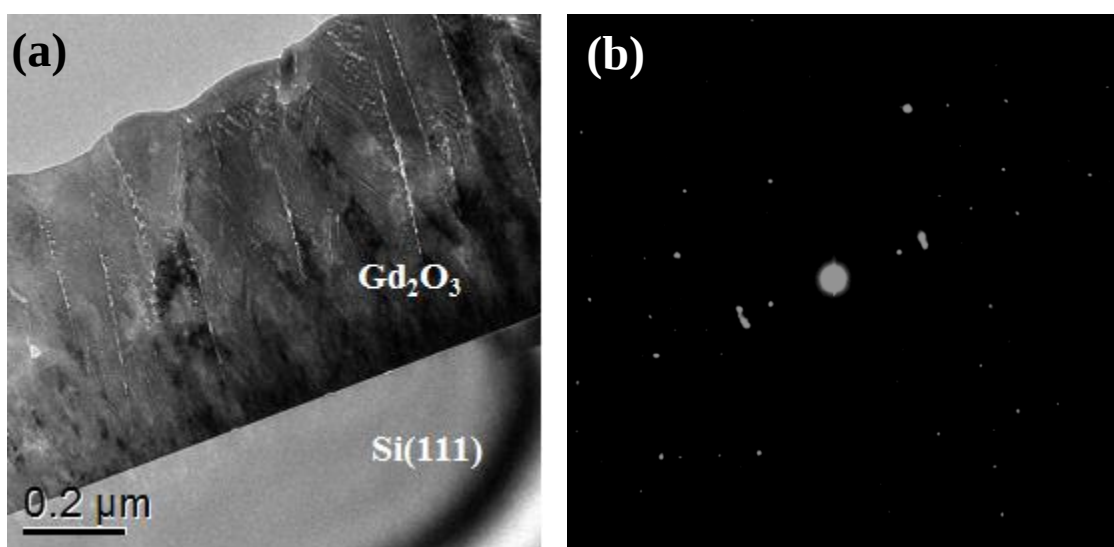
Figure 6.26. (a) Low-magnification bright-field image of thick \text{Gd}_2\text{O}_3 film (650 °C, 50 sccm \text{O}_2 , 1.01 \text{ μm} , 0.5 \text{ Å / s} ) deposited on silicon (111) and (b) corresponding SAD pattern collected from the film.
