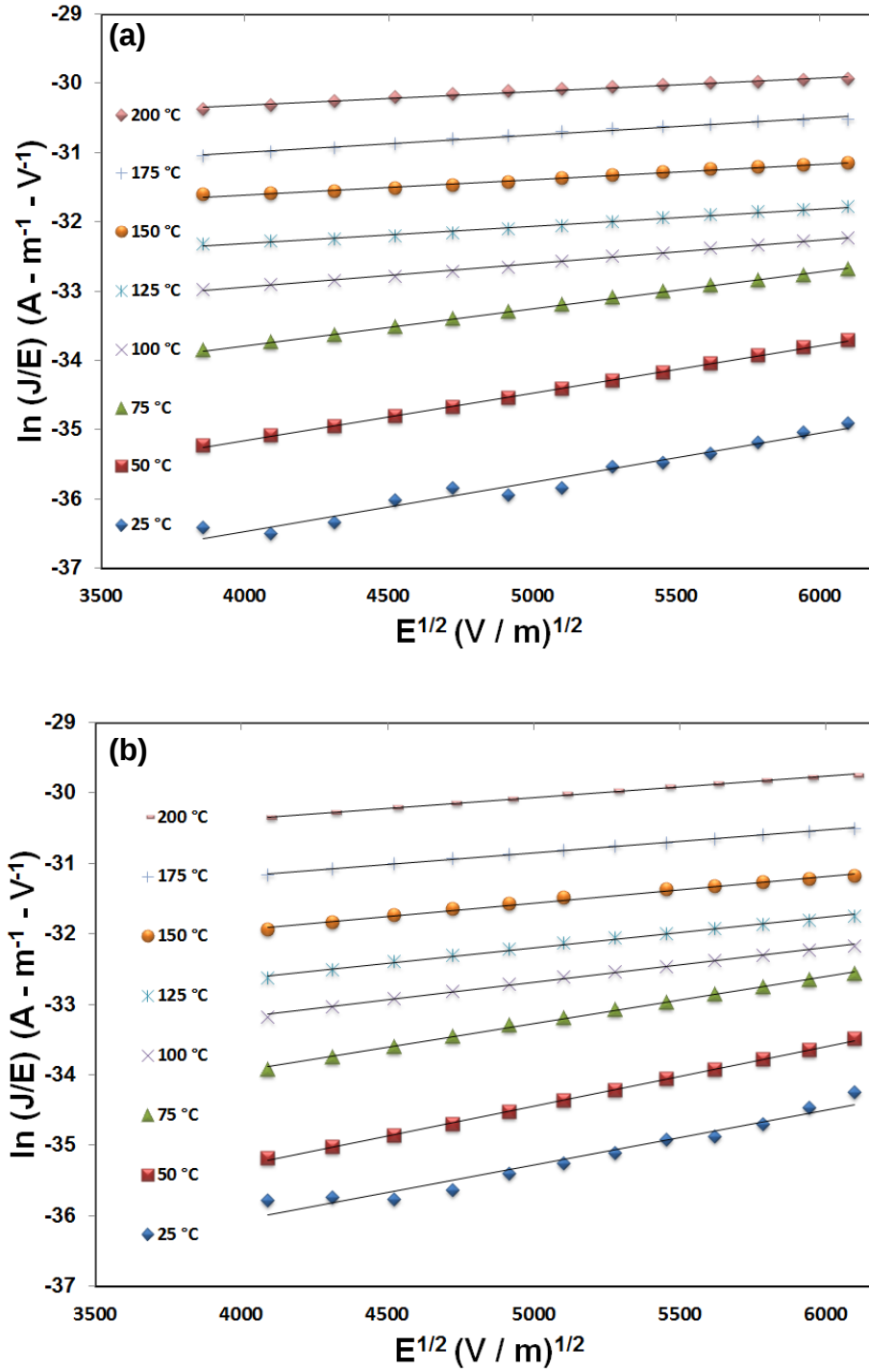
Figure 7.10. Poole-Frenkel plots ( \ln(J/E) vs E^{1/2} ) under (a) gate injection and (b) substrate injection for \text{Gd}_2\text{O}_3 film 9D (650 °C, 200 sccm \text{O}_2 , 2.69 \mu\text{m} ).
