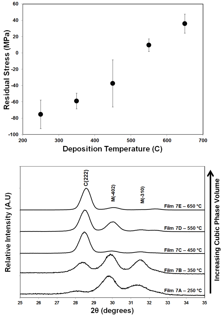
Figure 5.3. (a) Measured residual stress via wafer curvature technique for \sim 1 \mu\text{m} thick films 7A (250 °C), 7B (350 °C), 7C (450 °C), 7D (550 °C), and 7E (650 °C) deposited as a function of temperature on Si(111) under 50 sccm \text{O}_2 flow and (b) corresponding \theta -2 \theta diffraction patterns deposited on quartz substrates showing increasing cubic phase volume with increasing temperature.
