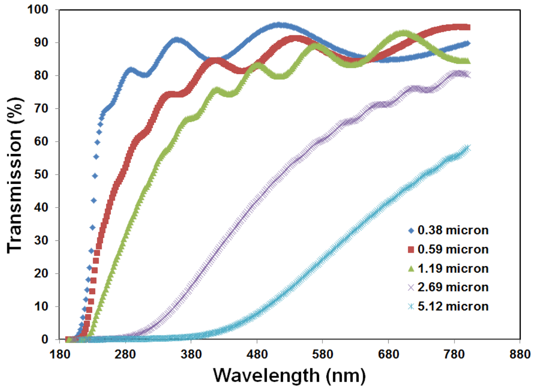
Figure B.2. UV-Vis transmission measurements for \text{Gd}_2\text{O}_3 films from set 9 (650 °C, 200 sccm \text{O}_2 , function of thickness) deposited on quartz.
