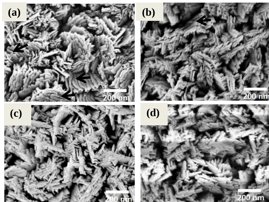
Figure 6.11. SEM top surface images of \text{Gd}_2\text{O}_3 films (a) 1A (50 sccm \text{O}_2 ), (b) 1B (100 sccm \text{O}_2 ), (c) 1C (150 sccm \text{O}_2 ), and (d) 1D (200 sccm \text{O}_2 ) deposited on silicon as a function of oxygen flow at 650 °C at high rates ( > 5 \text{ \AA} / \text{s} ). Arrows denote ridge-like growth.
