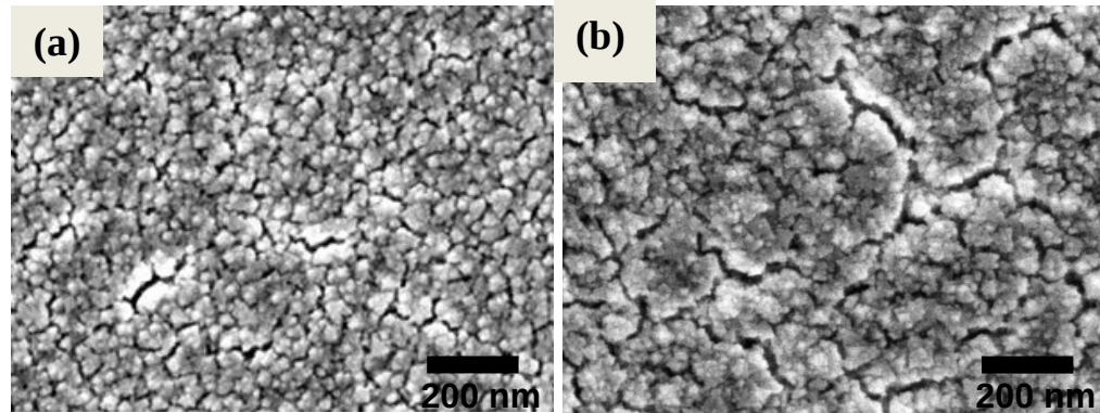
Figure 6.14. SEM surface images of film (a) 3A (580 nm) and (b) 3D (5.2 \mu\text{m} ) deposited on silicon at 250 °C under 200 sccm \text{O}_2 flow at high rates ( > 5 \text{ \AA} / \text{s} ).
